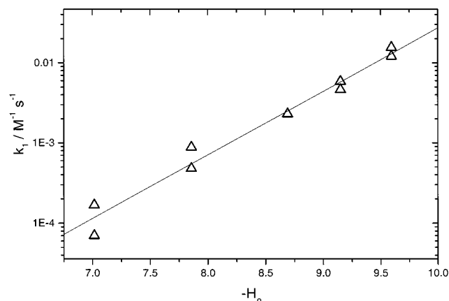
Figure 3. The second-order rate constant k_1 vs the sulfamic acid Hammett acidity function -H_0 at 306 K.
