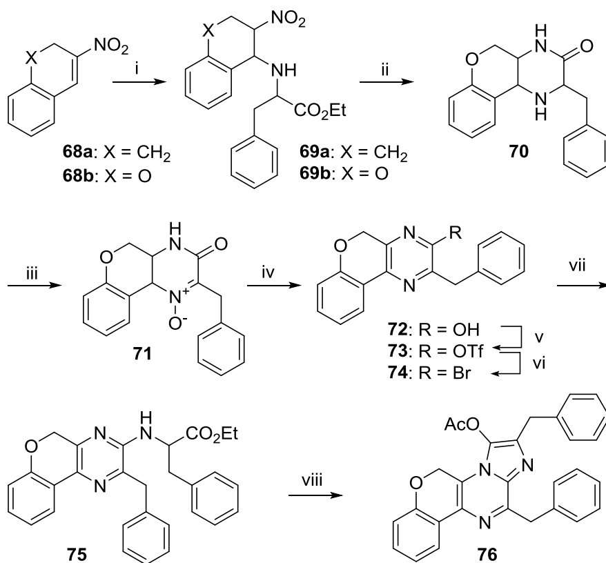
Scheme 9. i: PheOEt ( 23 ; free base), neat, 0 °C. ii: 1) Zn dust, 37% H 3 O + Cl - , dioxane, 0-20 °C, 2) neat, 140 °C. iii: 35% AcOOH/AcOH, AcOEt, 20 °C. iv: NaOH, EtOH, 20 °C. v: Tf 2 O, NEt 3 , CH 2 Cl 2 , 20 °C. vi: NaBr, TfOH, DMF, 120 °C. vii: PheOEt ( 23 ), Pd(OAc) 2 , BINAP, Cs 2 CO 3 , toluene, 85 °C. viii: 1) NaOH, THF, 20 °C, 2) Ac 2 O, 20 °C.
