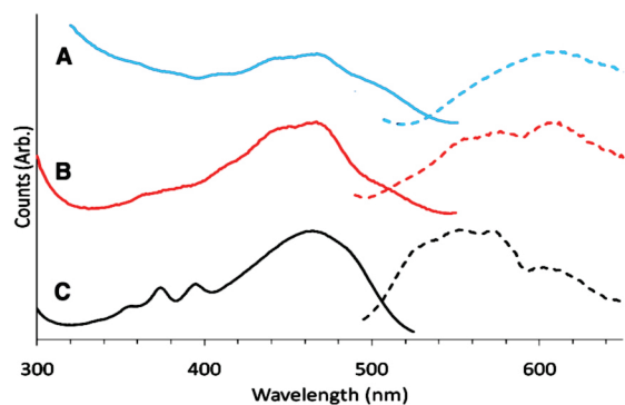
Figure 2. Excitation and emission spectra of dianthryl cyclopropenone 1g in CH 2 Cl 2 (C, black) and in an aqueous suspension (B, red). Excitation and emission spectra of dianthryl acetylene 2g in an aqueous suspension (A, blue).
