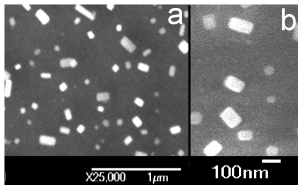
Figure 1. (a) SEM image of DPCP isolated nanocrystals showing crystals of ca. 50–200 nm on an alkane monolayer on a Si surface. (b) 4.6× magnification of the right portion of panel a.
