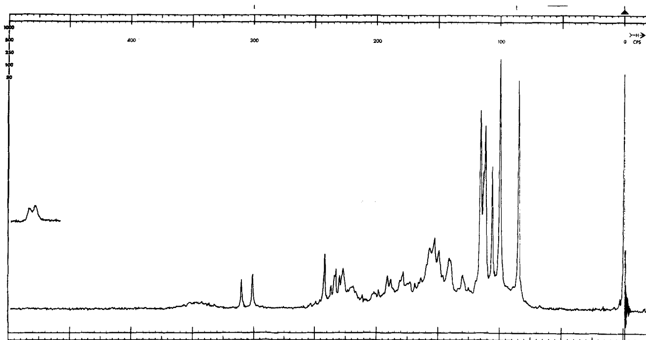
Figure 1—NMR spectrum of spiro -[5-androsten-3 \beta -ol-17-yl-5'-(N-ethyl-2',2'-dimethyloxazolidine)] (VIII).
