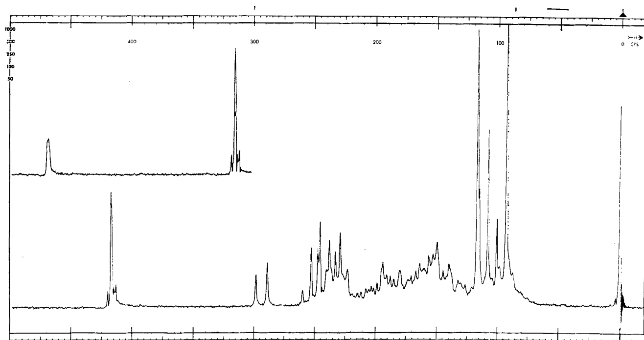
Figure 3—NMR spectrum of spiro-[4-androsten-3-one-17-yl-2'-(N-ethyloxazolidine)] (XVIII).
