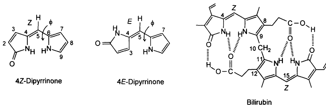
Figure 1. Naked unsubstituted dipyrinones in their 4 Z - and 4 E - configurations. (4 Z ,15 Z )-bilirubin-IX \alpha (bilirubin), which is composed of two Z -dipyrinones, each of which is intramolecularly hydrogen bonded to an opposing propionic acid. Hydrogen bonds are indicated by hatched lines.
