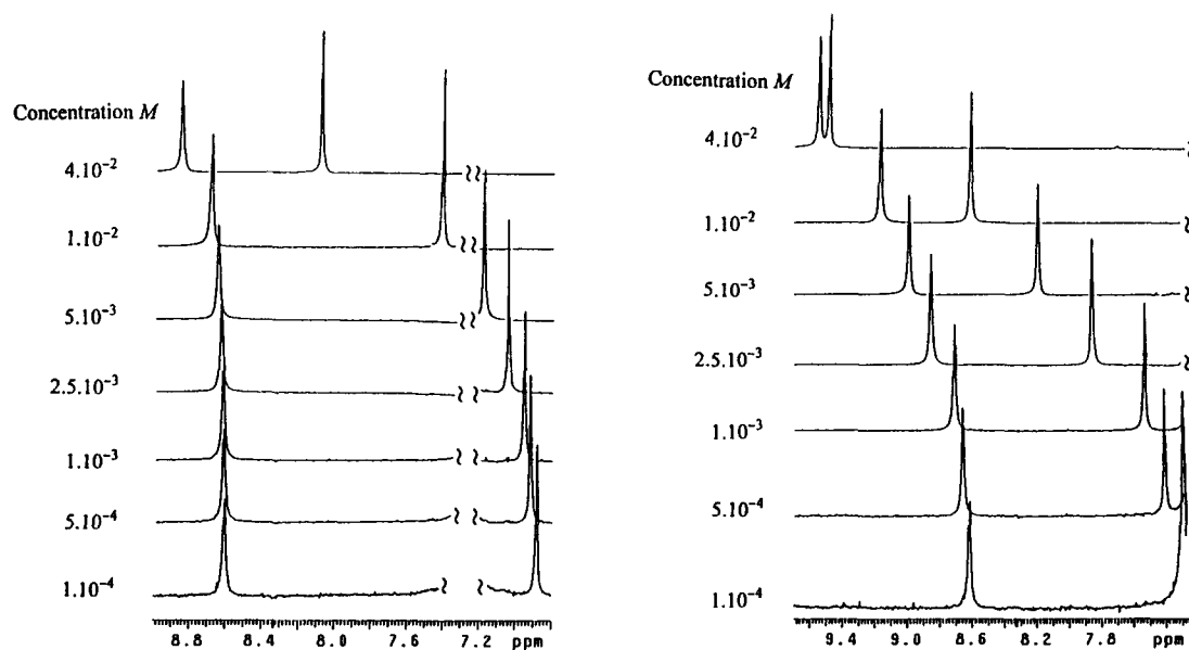
Figure 3. Partial ^1\text{H} -NMR spectra showing concentration dependence in CDCl 3 solvent of the dipyrinone lactam and pyrrole NH chemical shifts of ( E )-3 (left) and ( Z )-3 (right). The lactam NH is more shielded in ( E )-3, but more deshielded in ( Z )-3.
