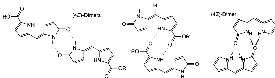
Figure 4. Intermolecularly hydrogen-bonded dipyrinone dimers.
