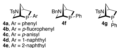
Figure 2. HypPhos catalysts 4.
