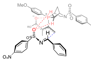
Figure 3. Proposed transition state for the [4 + 2] annulation of 5 and 6a .
