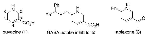
Figure 1. Guvacine and bioactive guvacine derivatives.
