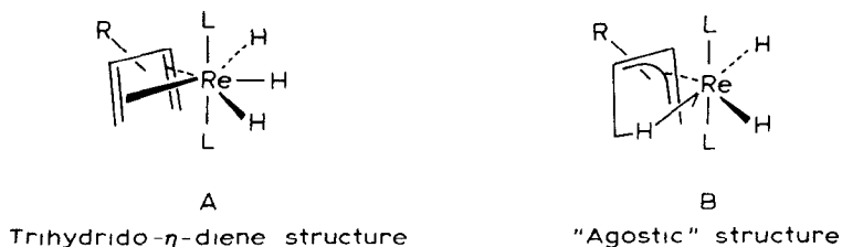
Fig. 1. Possible structures of the rhenium complexes I-V ( L = \text{Ph}_3\text{P} )
