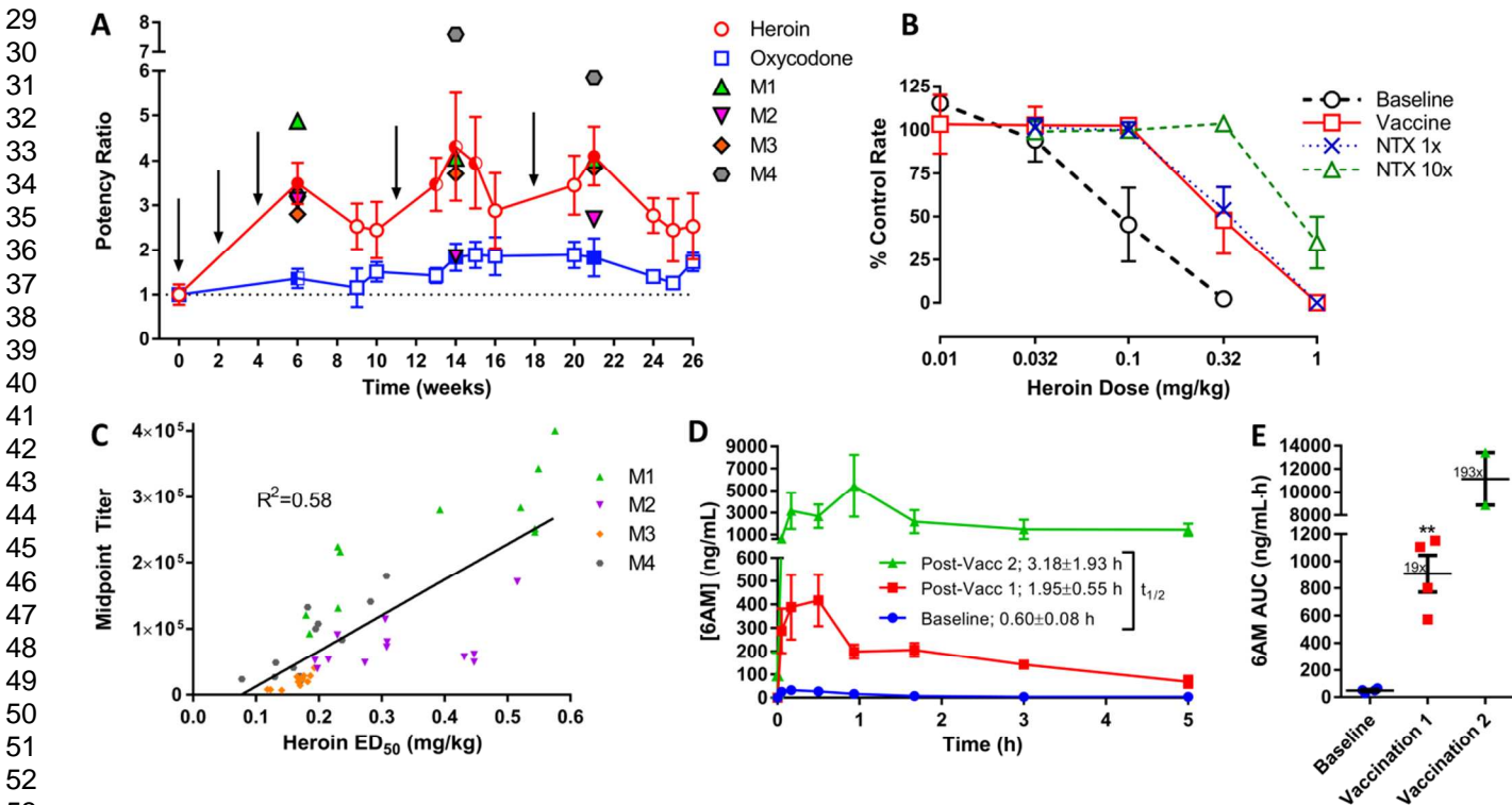
Figure 6. Heroin vaccine diminishes heroin potency and alters 6AM pharmacokinetics in rhesus monkeys. (A) Timeline of changes in either heroin or oxycodone ED 50 in monkeys after heroin vaccine administration. Monkeys (M1-4) were vaccinated i.m. at the indicated time points (arrows) with 400 \mu g HerCOOH-TT, 600 \mu g CpG ODN 2006 and 5 mg alum. Baseline heroin and oxycodone ED 50 values were double-determined in each monkey prior to vaccination in the assay of schedule-controlled responding (SCR). Each point in the figure represents the average ratio of heroin (red) or oxy (blue) ED 50 \pm SEM relative to the baseline value. Group mean \pm SEM baseline ED 50 values for heroin and oxycodone were 0.08 \pm 0.03 and 0.19 \pm 0.06 mg/kg, respectively. RM one-
