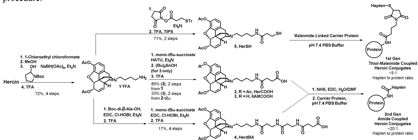
Scheme 1. Synthesis and conjugation of heroin haptens.
