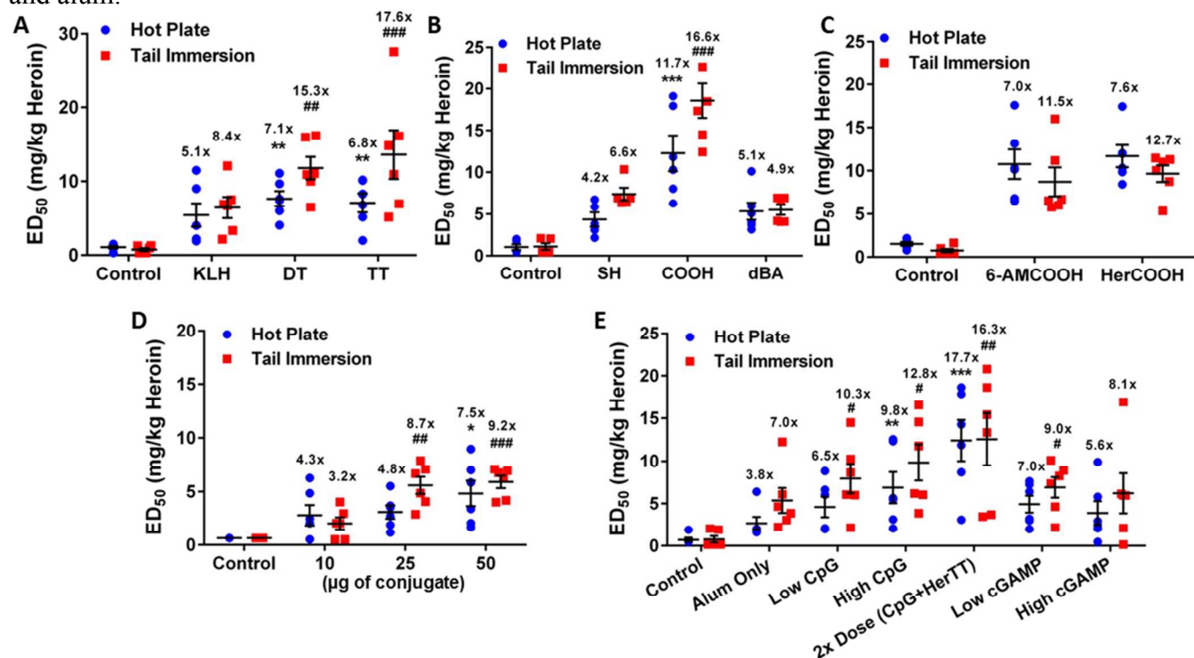
Figure 3. Optimization of heroin immunoconjugate and vaccine formulation. (A) Comparison of carrier proteins with HerSH hapten. ## P < 0.01 , ### P < 0.001 , ** P < 0.01 versus KLH. (B) Evaluation of heroin haptens as TT immunoconjugates. ### P < 0.001 , *** P < 0.001 versus HerSH-TT. (C) Comparison study of 6AMCOOH vs. HerCOOH haptens as TT conjugates. (D) Dose-dependency of HerCOOH-TT immunoconjugate on vaccine efficacy. ## P < 0.01 , ### P < 0.001 , * P < 0.05 versus 10 \mu\text{g} dose. No CpG ODN was used. (E) Adjuvant effects of CpG ODN 1826 and cGAMP on vaccine efficacy. Doses: 4 \mu\text{g} CpG (Low CpG), 30 \mu\text{g} CpG (High CpG), 60 \mu\text{g} CpG + 100 \mu\text{g} HerCOOH-TT (2X dose), 1.3 \mu\text{g} (Low cGAMP), 10 \mu\text{g} (High cGAMP). # P < 0.05 , ## P < 0.01 , ** P < 0.01 , *** P < 0.001 versus alum only. Vaccine formulations for all panels contained 0.75 mg alum, 30 \mu\text{g} CpG ODN 1826 and 50 \mu\text{g} HerCOOH-TT unless otherwise noted and were administered to n = 6 mice i.p. at wk 0, 2 and 4. For all panels, the mean heroin \text{ED}_{50} \pm \text{SEM} (determined via cumulative s.c. dosing) is shown and statistics were evaluated by a one-way ANOVA with Tukey's post-hoc test. Testing was performed at wk 6 and significance is denoted by (#) for tail immersion and (*) for hot plate. Fold-shifts in \text{ED}_{50} versus n = 6 non-vaccinated control mice are reported above each set of data points.
