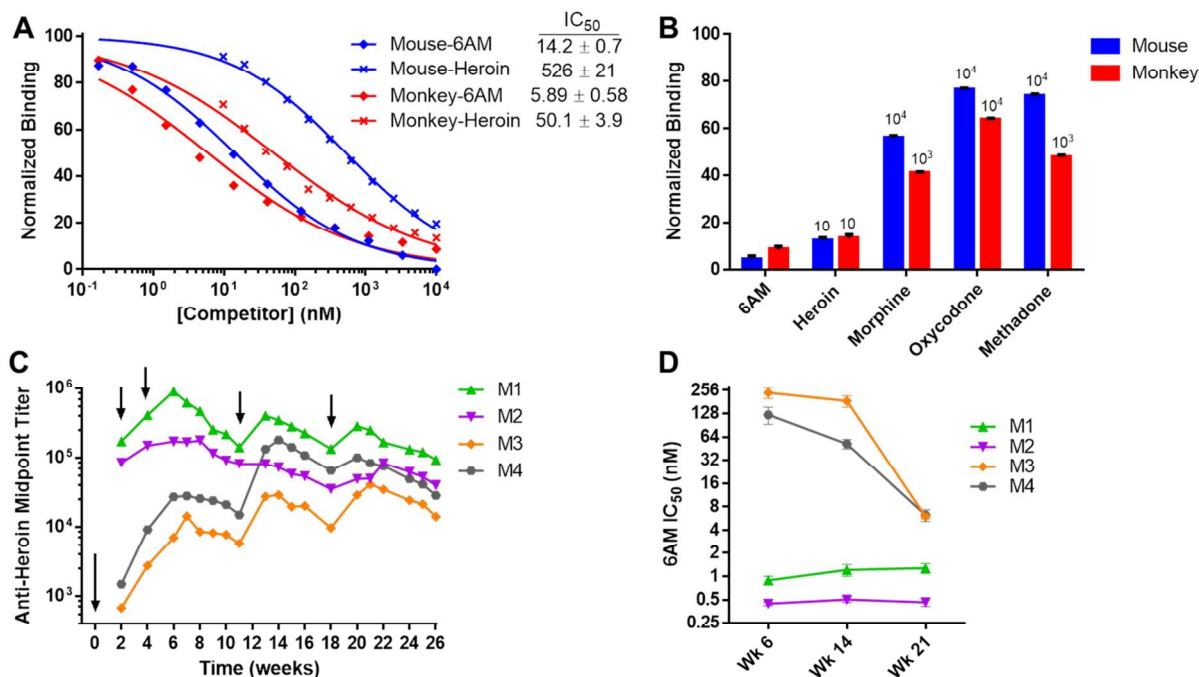
Figure 5. Heroin conjugate vaccine elicits a robust anti-drug antibody response in monkeys with high affinity and selectivity for 6AM. (A) Binding curves of vaccinated monkey and mouse antiserum for heroin and 6AM as determined by SPR in triplicate. Points represents the mean binding to immobilized HerCOOH-BSA following serum incubation with 12 dilutions of heroin or 6AM competitors. Binding values were normalized to serum binding without competitor drug. Listed IC_{50} s \pm SEM were derived from a nonlinear fit of the binding curves. Serum was pooled from n = 2 monkeys (M1,2) and n = 6 mice collected after three initial immunizations. (B) Binding selectivity of mouse and monkey antiserum for various opioids at 100 \mu M ([6AM] = 10 \mu M) by SPR in triplicate. Minimum selectivity factors relative to 6AM are shown above each bar. (C) Anti-heroin IgG titers of rhesus monkeys (M1-4) vaccinated at the indicated time points (arrows) with 400 \mu g HerCOOH-TT, 600 \mu g CpG ODN 2006 and 5 mg alum. Midpoint titers were determined in duplicate by ELISA against a HerCOOH-BSA coating antigen. No anti-heroin IgM titers were detected at any point. Monkeys M1 and M2 were previously vaccinated with the heroin vaccine in a pilot study while M3 received unconjugated TT. M4 was not pretreated. (D) Individual monkey antiserum affinity for 6AM over time by SPR. Points represent mean IC_{50} \pm SEM determined from a 12 point 6AM dilution curve similar to panel A methods. Time points match up with the panel C timeline.
