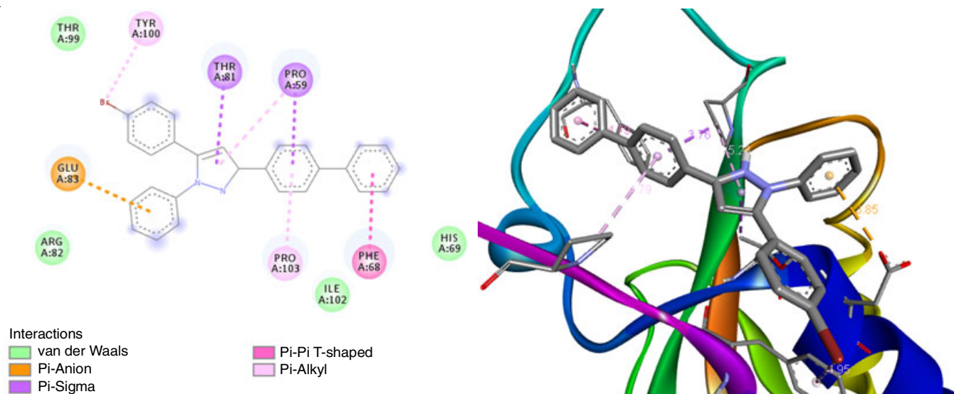
Fig. 2. 2D and 3D image of compound 4,5-dihydro-1-phenyl-3-diphenyl-5-(4-bromophenyl)-1 H -pyrazole ( 2d ) docked with breast cancer protein (10QA)
