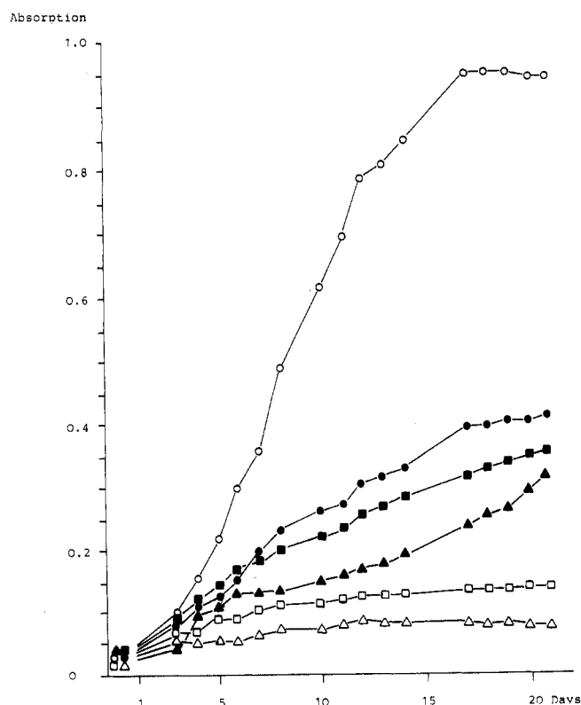
Figure 2. Growth inhibition of M. tuberculosis H 37 Ra by 93: 32 μg/mL (Δ), 16 μg/mL (□), 8 μg/mL (▲), 4 μg/mL (■), 2 μg/mL (●); control (○); Middlebrook 7H9 medium (liquid); turbidimetric measurement at 546 nm.
