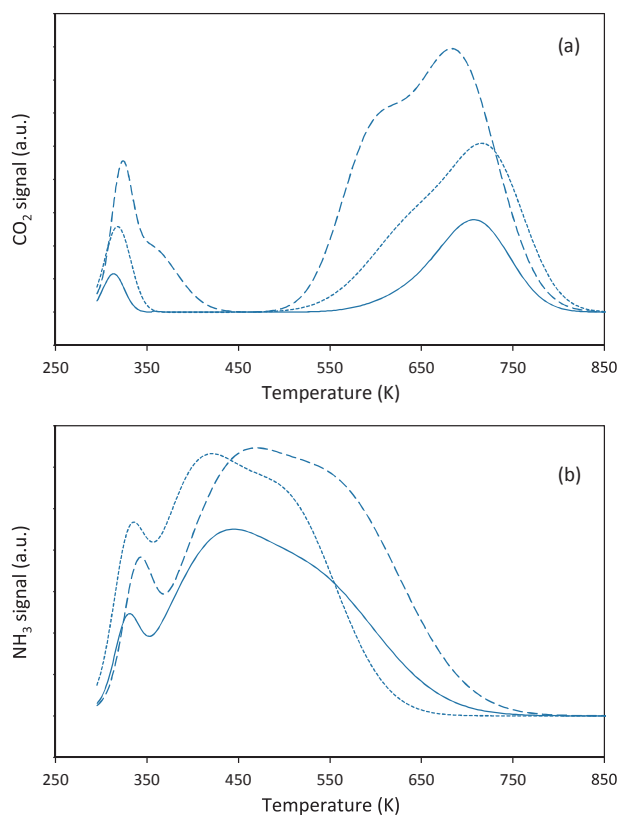
Fig. 1. Characterization of basicity and acidity: (a) CO 2 -TPD; (b) NH 3 -TPD. Symbols: P25 (continuous line); mP25 (long dashes); AumP25 (dotted line).
