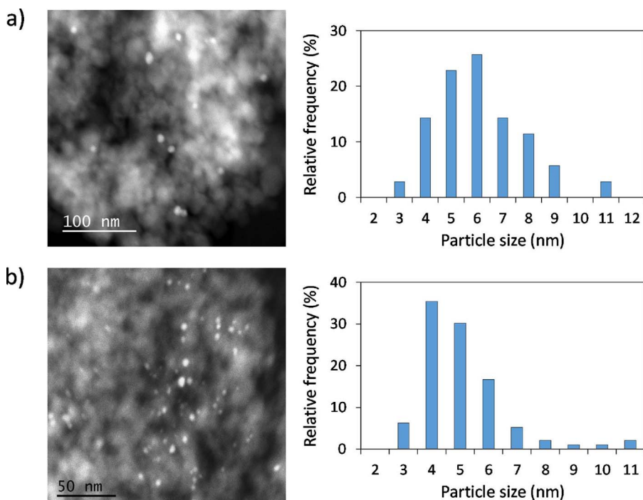
Fig. 8. STEMHAADF images and gold nanoparticle distributions of the spent catalysts recovered after 8 h of reaction under inert conditions at 673 K: (a) Au/mTiO 2 , and (b) Au/SiO 2 .
