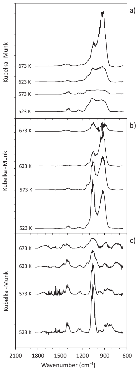
Fig. 9. DRIFT spectra in the gas phase ethanol condensation under reductive conditions over: (a) \text{TiO}_2 , (b) \text{mTiO}_2 , and (c) \text{Au/mTiO}_2 .
