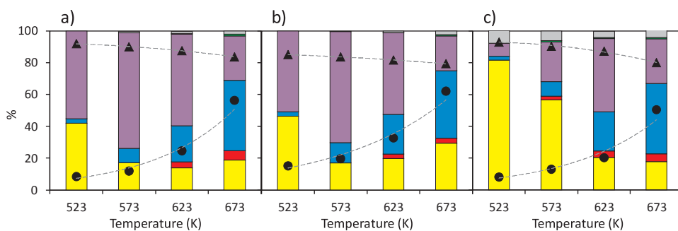
Fig. 6. Conversion, carbon balance, and selectivity evolution in the gas phase ethanol condensation under inert conditions over: (a) \text{TiO}_2 , (b) \text{mTiO}_2 , and (c) \text{Au/mTiO}_2 . (WHSV = 7.9 \text{ h}^{-1} ; He flow). Symbols: conversion (●), carbon balance (▲). Bars: acet-aldehyde (yellow), ethylene (blue), diethyl ether (purple), 1butanol (red), 1,3butadiene (green), and others (grey). (For interpretation of the references to colour in this figure legend, the reader is referred to the web version of this article.)
