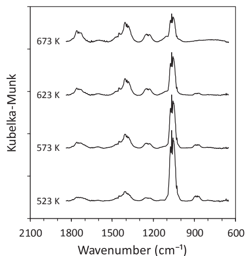
Fig. 10. DRIFT spectra in the gas phase ethanol condensation over \text{Au/mTiO}_2 under inert conditions.
