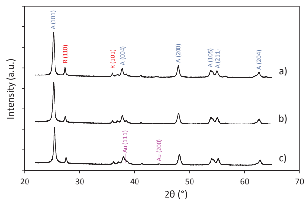
Fig. 2. XRD diffractograms of (a) TiO 2 , (b) mTiO 2 , and (c) Au/mTiO 2 . Corresponding peak's crystalline phase: A, anatase; R, rutile; Au, gold; planes in brackets.
