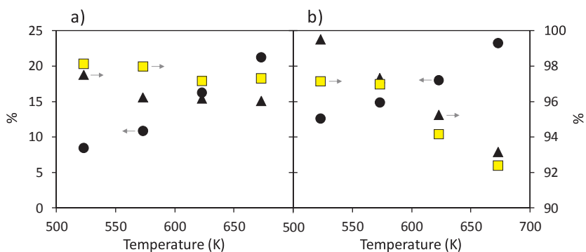
Fig. 7. Conversion (●), carbon balance (▲), and acetaldehyde selectivity (■) evolution in the gas phase ethanol condensation over \text{Au/SiO}_2 under: (a) reductive conditions ( \text{He-H}_2 flow), and (b) inert conditions (He flow). (WHSV = 7.9 \text{ h}^{-1} ).
