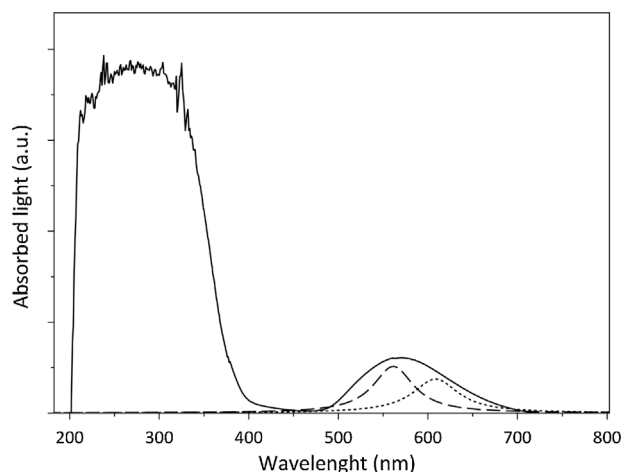
Fig. 4. Diffusereflectance UVVis spectra of the Au/ \text{mTiO}_2 catalyst (dashed lines: deconvolution of the gold SPR absorption band).
