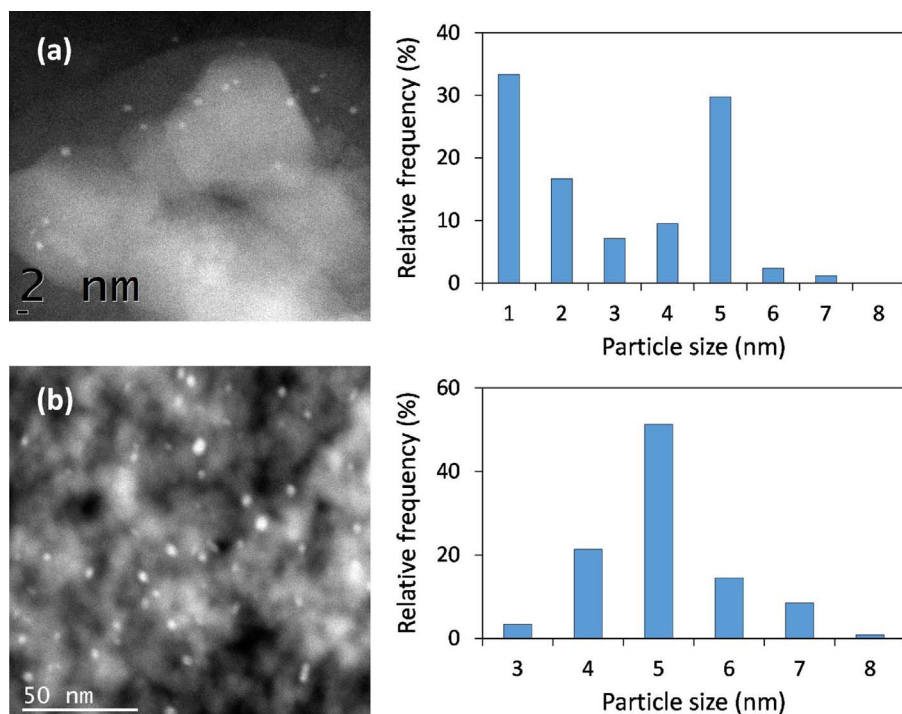
Fig. 3. STEMHAADF image of the (a) Au/ \text{mTiO}_2 and (b) Au/ \text{SiO}_2 materials. Analysis of gold particle size distribution.
