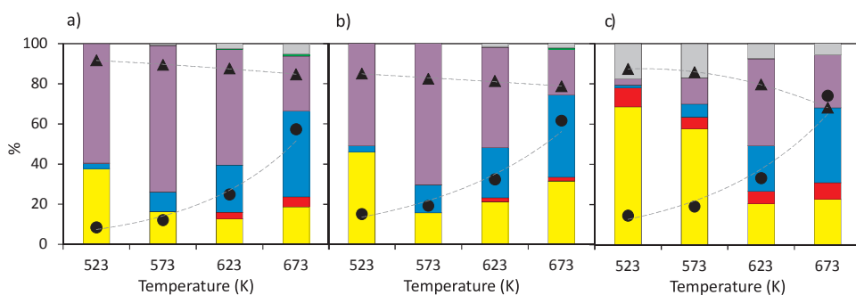
Fig. 5. Conversion, carbon balance, and selectivity evolution in the gas phase ethanol condensation under reducing conditions over: (a) TiO 2 , (b) mTiO 2 , and (c) Au/mTiO 2 . (WHSV = 7.9 h -1 ; He-H 2 flow). Symbols: conversion (●), carbon balance (▲). Bars: acetaldehyde (yellow), ethylene (blue), diethyl ether (purple), 1butanol (red), 1,3butadiene (green), and others (grey). (For interpretation of the references to colour in this figure legend, the reader is referred to the web version of this article.)
