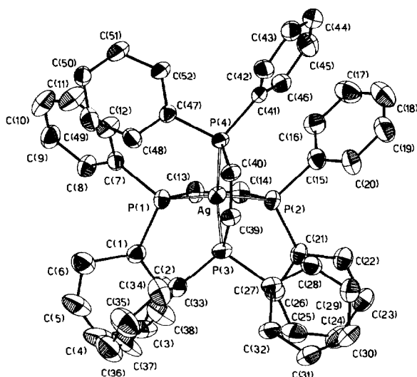
Fig. 1. Perspective view of the [Ag(cdppt)_2]^+ cation.
