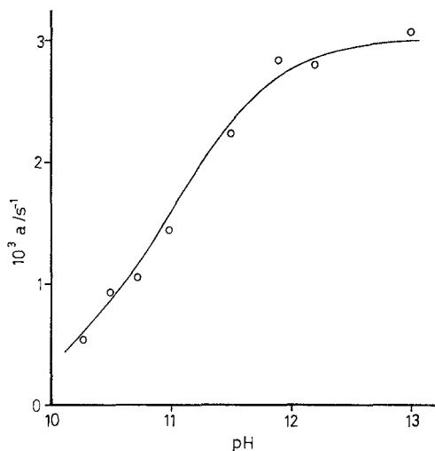
Fig. 3. Effect of pH on the parameter a at 25^\circ C , I = 0.25 M , [PrONO] = 3.3 \cdot 10^{-4} M [DMA] = 4.47 \cdot 10^{-2} M
