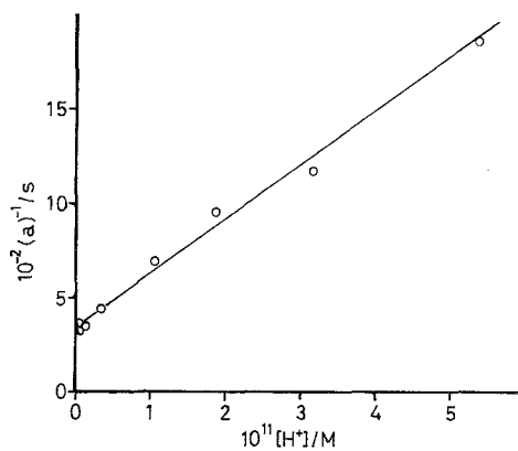
Fig. 4. The parameter a^{-1} plotted against [H^+] at 25^\circ C , I = 0.25 M , [PrONO] = 3.3 \cdot 10^{-4} M and [DMA] = 4.47 \cdot 10^{-2} M
