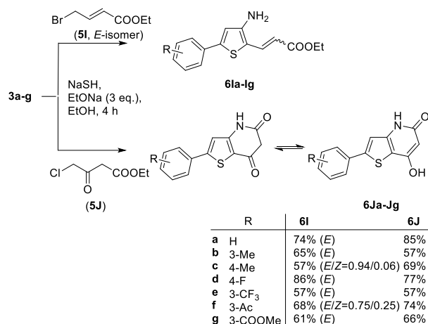
Scheme 7. Formation of thiophenes 6 by three-component reactions.
