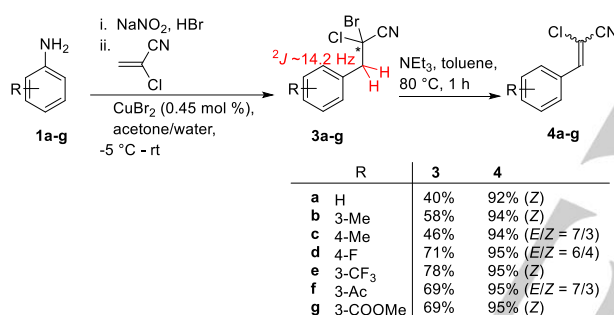
Scheme 4. Syntheses of propanenitriles 3 and 2-chlorocinnamionitriles 4 .
