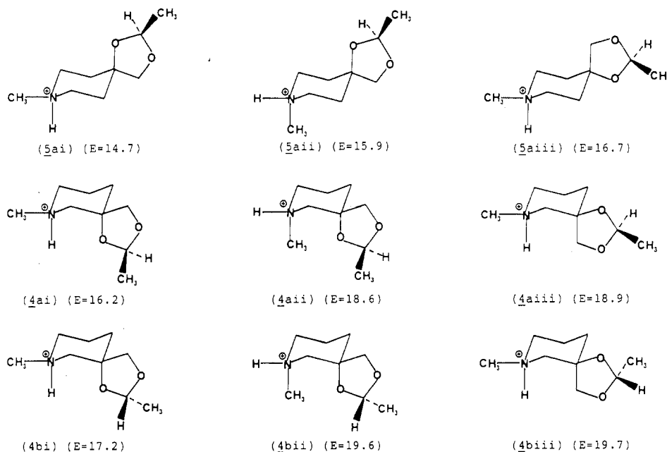
Figure 3. Lowest energy forms of 4a , 4b , and 5a from molecular mechanics calculations. All conformations of each isomer were considered in the analysis, but those not displayed had significantly higher energy. The relative stereochemistry of 4a and 4b has been arbitrarily assigned. No comparison of absolute energies between 4a , 4b , and 5a is intended. Figures in brackets are calculated energies in kcal Mol -1 .
