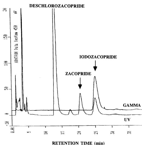
Fig. 1. Chromatogram of [ 125 I]iodination of Deschloro-( S )-zacopride Using a Reverse-phase Cyano Column in 44% MeCN in 20 mM Phosphate Buffer as the Mobile Phase
