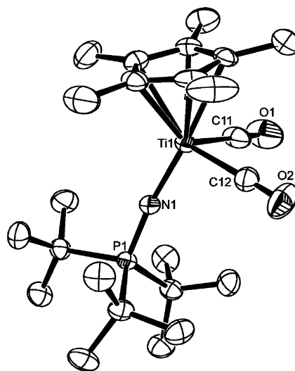
Figure 13. ORTEP drawings of one of the two molecules of 22 in the asymmetric unit, 30% thermal ellipsoids are shown. Hydrogen atoms are omitted for clarity. Distances (Å) angles (deg): Ti(1)–N(1) 1.841(2), Ti(1)–C12 2.021(3), Ti(1)–C11 2.028(4), Ti(1)–C5 2.341(3), Ti(1)–C(4) 2.352(3), Ti(1)–C(1) 2.366(3), Ti(1)–C(3) 2.403(3), Ti(1)–C(2) 2.413(3), P(1)–N(1) 1.586(2), C(11)–O(1) 1.150(4), C(12)–O(2) 1.146(3), N(1)–Ti(1)–C(12) 97.82(11), N(1)–Ti(1)–C(11) 100.42(11), C(12)–Ti(1)–C(11) 88.07(14), P(1)–N(1)–Ti(1) 172.30(14), O(1)–C(11)–Ti(1) 179.2(3), O(2)–C(12)–Ti(1) 178.1(3), N(1)–Ti(1)–C(12) 97.82(11), N(1)–Ti(1)–C(11) 100.42(11).
