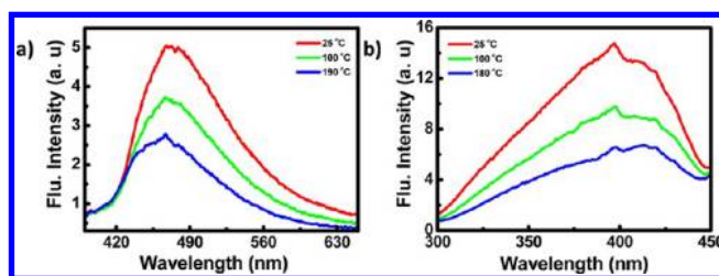
Figure 7. Temperature dependent changes on (a) emission spectra ( \lambda_{\text{exc.}} = 350 nm) and (b) excitation spectra (emission collected at 475 nm) of FD16 .
