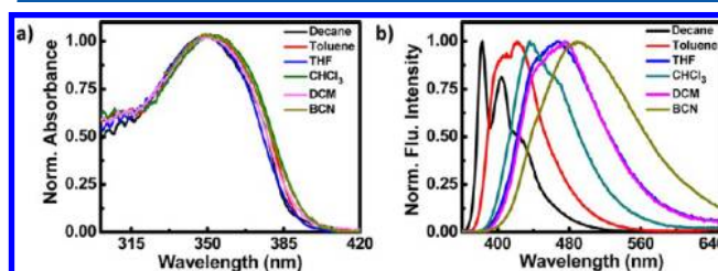
Figure 6. (a) Absorption and (b) emission spectra of FD12 in different solvents.
