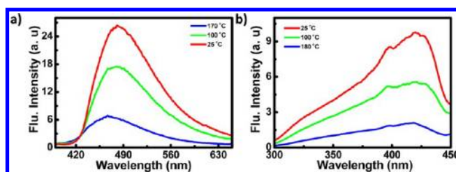
Figure 8. Temperature dependent changes on (a) emission spectra ( \lambda_{\text{exc.}} = 350 nm) and (b) excitation spectra (emission collected at 475 nm) of FD12 .
