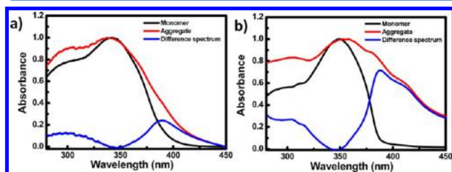
Figure 11. Difference spectra (blue line) of (a) FD12 and (b) FD16 obtained by subtracting the absorption spectrum of monomer (black line) from absorption spectrum of completely aggregated solution (red line).
