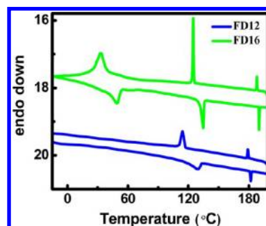
Figure 2. DSC thermogram of FD16 and FD12 .
