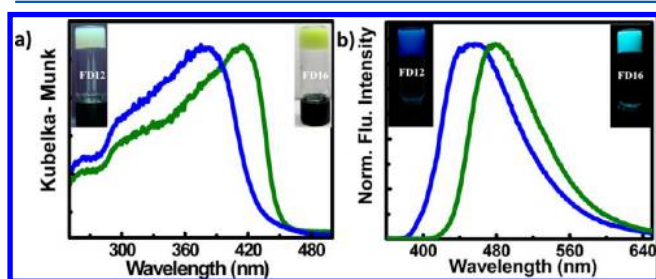
Figure 15. (a) Absorption and (b) emission spectra of FD12 (blue line), FD16 (green line) in gel ( \lambda_{\text{ex}} = 350 nm; 2 \times 10^{-2} M in decane; 1 mm cuvette). Inset shows the corresponding photographs of gel under white light and 365 nm UV illumination.
