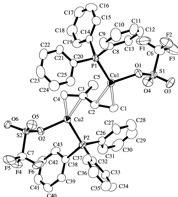
Fig. 1. View of [\text{Cu}_2(\text{PPh}_3)_2\{\mu\text{-(H}_2\text{C=CHC(CH}_3\text{)=CH}_2\text{)}\}(\text{O}_3\text{SCF}_3)_2] ( 1 ), showing the crystallographic numbering. Thermal ellipsoids enclose 50% probability. In addition, Cu(1) is coordinated by O(3) of a neighbouring triflate group and Cu(2) likewise by O(6) of a neighbouring triflate ligand (see Table 3).
