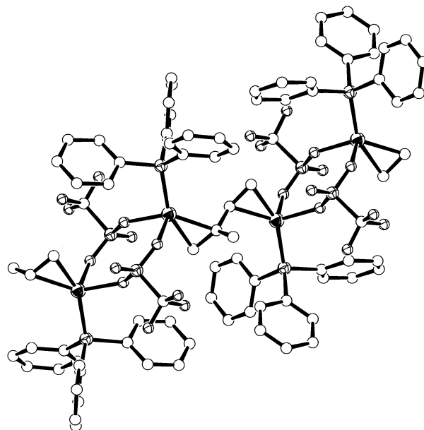
Fig. 2. Part of a chain in [\text{Cu}_2(\text{PPh}_3)_2\{\mu\text{-(H}_2\text{C=CHC(CH}_3\text{)=CH}_2\text{)}\}(\text{O}_3\text{SCF}_3)_2] ( 1 ), showing the alternate bridging of copper(I) by isoprene and triflate (participating in eight-membered \text{Cu}_2\text{S}_2\text{O}_4 rings).
