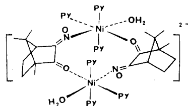
Figure 2. The dimeric structure of [Ni(CQM)(py) 3 (H 2 O)]PF 6 ·H 2 O.
