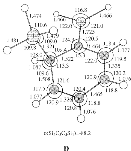
Figure 4. Calculated RHF/6-31G** geometries of silene arising from a 1,3-silyl shift ( D ). All bond lengths are in angstroms and all angles are in degrees.
