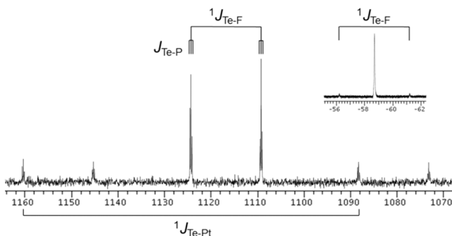
Figure 6. ^{125}\text{Te} NMR spectrum of 4 in \text{CDCl}_3 . The inset shows the ^{19}\text{F} NMR spectrum.
