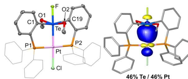
Figure 7. Left: Solid-state structure of 4 . Thermal ellipsoids are drawn at the 50% probability level. Phenyl groups are drawn in wireframe. Hydrogen atoms and solvent molecules are omitted for clarity. Pertinent metrical parameters can be found in the text. Right: NLMO plot (isovalue = 0.05) of the Te–Pt bond in 4 obtained from NBO analysis. Hydrogen atoms are omitted for clarity.
