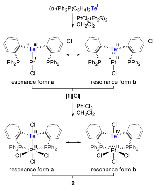
Scheme 1. Synthesis of [1][Cl] and 2
