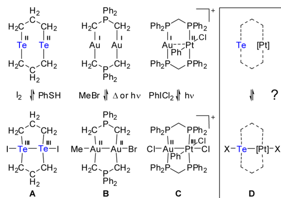
Chart 1. Two-Electron Redox Processes in Selected Dinuclear Complexes
