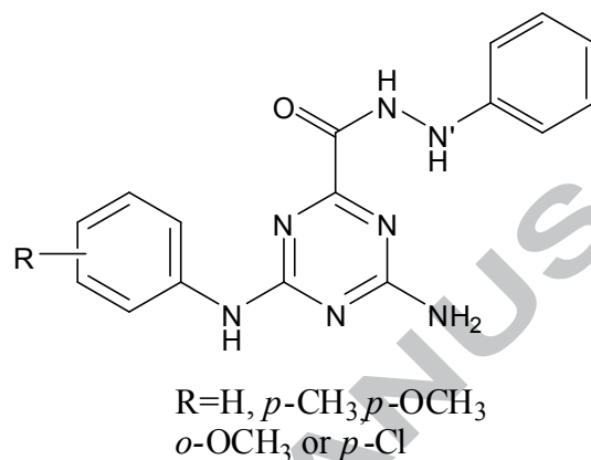
Fig.2: 4-amino-N'-phenyl-6-(arylamino)-1,3,5-triazine-2-carbohydrazides
