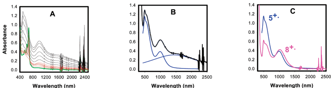
Figure 3. A. Spectral changes upon the reduction of 1.1 \times 10^{-4} M 9 + (green) in dichloromethane at 22 °C by incremental addition of 4.7 \times 10^{-3} M 5 to give first 5 3+ (red) and then 5 + (black) upon further additions of neutral 5 . B. Plot of deconvoluted spectra of 5 + . C. Similarity in the UV-vis region of the spectrum of the cation radical 5 + (blue, partial spectrum obtained by deconvolution) with that of the model 8 + (magenta).
