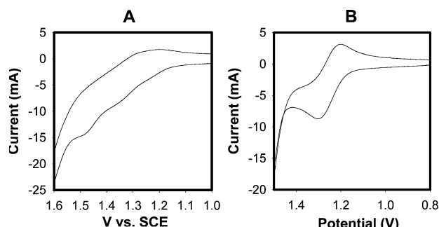
Figure 2. Cyclic voltammograms of 2 mM hexakis(4-tetraphenylethylene)benzene 5 (A) and model donor 8 (B) in CH 2 Cl 2 containing 0.2 M tetra- n -butylammonium hexafluorophosphate at a scan rate of 200 mV s -1 and at 22 °C.
