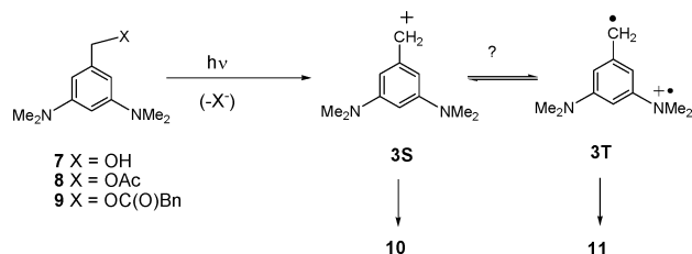
Scheme 4. Photoheterolysis Mechanism
