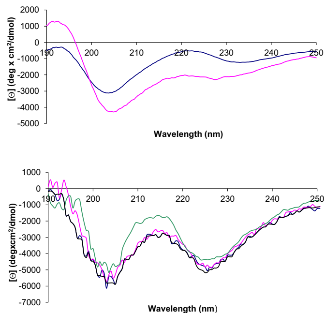
Fig. 7. CD spectra of peptide 1 , top, in PBS buffer (pH=7), blue line, and with 25% TFE added, purple line, and tripodal template 2 , bottom, in PBS buffer, black line, with 56% TFE, blue line, 72% TFE, purple line, and 100% TFE, green line.
