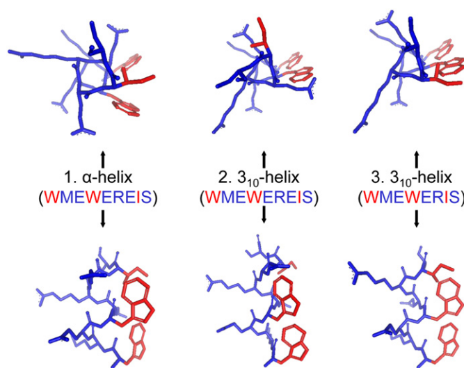
Fig. 3. The relevant sequence imposed on an \alpha -helix (1), a 3 10 -helix (2) and the same sequence in which one residue between W (Trp) and I (Ile) is eliminated imposed on a 3 10 -helix (3). WWI-residues in red. Helical conformations are reported with canonical torsion angles.
