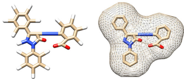
FIGURE 3 Optimized molecular structure of 2-((5-oxo-1,3-diphenyl-4,5-dihydro-1H-pyrazol-4-yl)diazanyl) benzoic acid (HL)
