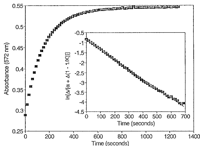
Figure 1. Representative absorbance vs time plot for reaction 3. [(\text{TTP})\text{Ti}=\text{O}]_0 = 1.95 \times 10^{-5} \text{ M} and [(\text{OEP})\text{TiCl}]_0 = 1.94 \times 10^{-5} \text{ M} , in toluene at 20^{\circ}\text{C} . Inset shows plot of \ln[\Delta/(\alpha + \Delta(1 - 1/K))] vs t , k_f = 240 \pm 20 \text{ M}^{-1} \text{ s}^{-1} .
