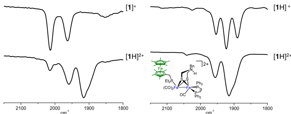
Figure 8. IR spectra for the generation of [1H]^{2+} : (left) by protonation of [1]^+ with 1 equiv of [H(OEt_2)_2]BARF_4 ; (right) by oxidation of [1H]^+ with 1 equiv of [Fc]BARF_4 . Inset: structure of [1H]^{2+} .
