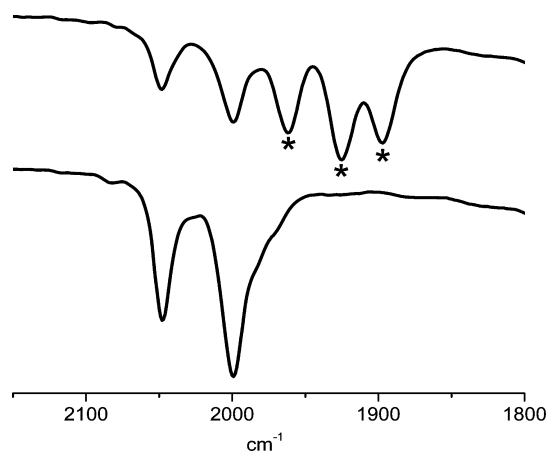
Figure 12. IR spectrum (CH 2 Cl 2 solution) of 3 in the presence of 5 equiv of [H(OEt)_2]BARF_4 at −15 °C: (top) after 40 min; (bottom) after 150 min. Peaks marked with asterisks are assigned as [3H]^+ .
