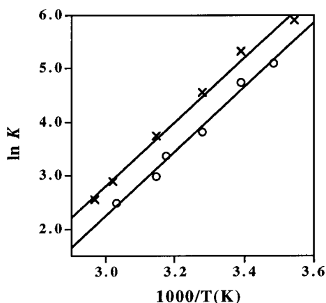
Figure 1. van't Hoff plots for the reaction of 21 with dibenzylamine to form 24 (denoted by x) and reaction of tert -octylamine with 21 to form 25 (denoted by o).
