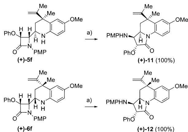
Scheme 6. Sodium methoxide promoted transformation of quinoline-β-lactams into enantiopure fused tricyclic indolizidinones. Reagents and conditions: a) MeONa, MeOH, room temperature, 16 h.
