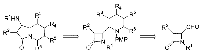
Scheme 1. Retrosynthetic analysis of indolizidine-type systems from 4-oxoazetidine-2-carbaldehydes.
