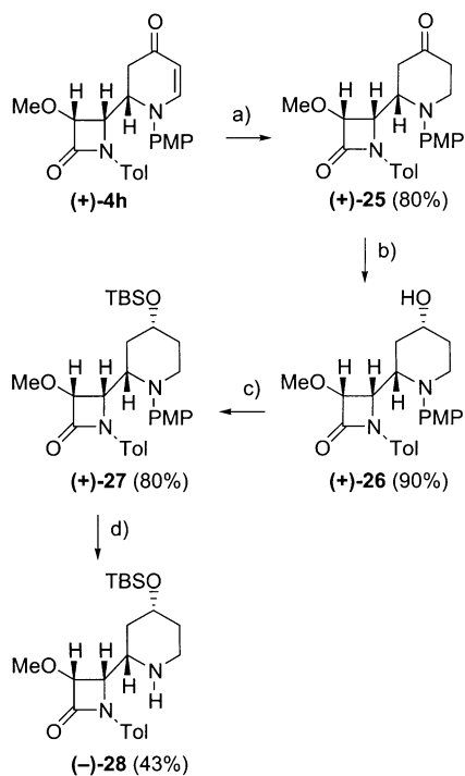
Scheme 9. Preparation of oxoazetidyl-piperidine ( (-)-28 ). Reagents and conditions: a) L-Selectride, THF, -78^{\circ}\text{C} , 1 h. b) \text{NaBH}_4 , MeOH, 0^{\circ}\text{C} . c) TBSCl, imidazole, DMF, room temperature. d) CAN, \text{CH}_3\text{CN}/\text{H}_2\text{O} , -35^{\circ}\text{C} .
