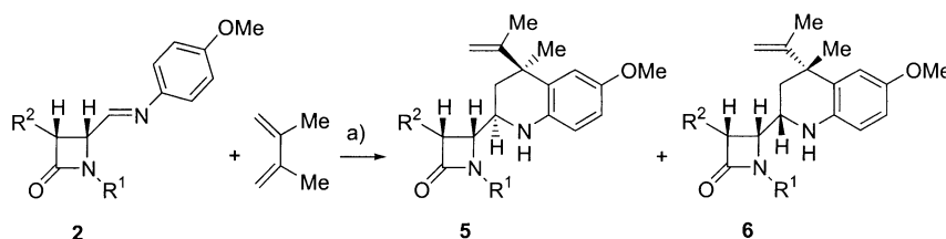
Scheme 4. Lewis acid-mediated Diels–Alder cycloaddition between 2-azetidinone-tethered imines and 2,3-dimethyl-1,3-butadiene. Reagents and conditions: a) Lewis acid, acetonitrile, room temperature.
