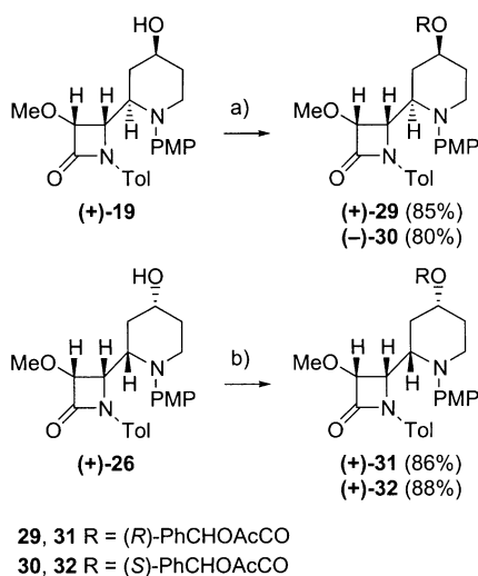
Scheme 10. Synthesis of acetylmandelates 29–32 . Reagents and conditions: a) ( R )-acetylmandelic acid, DCC, DMAP, dichloromethane, room temperature. b) ( S )-acetylmandelic acid, DCC, DMAP, dichloromethane, room temperature.
