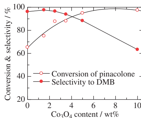
Figure 3. Influence of \text{Co}_3\text{O}_4 content in the \text{Co}_3\text{O}_4/\text{Al}_2\text{O}_3 catalyst on the average conversion of pinacolone at 425 °C.
