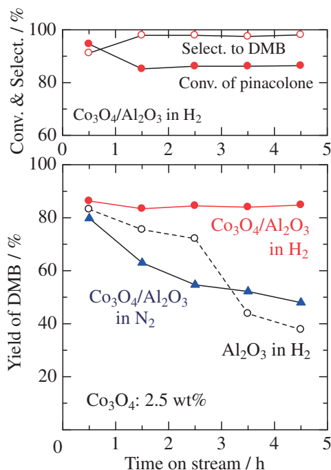
Figure 2. Change in the conversion of pinacolone over \text{Co}_3\text{O}_4/\text{Al}_2\text{O}_3 at 425 °C with time on stream.
