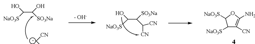
Proposed mechanism for the formation of compound 4
