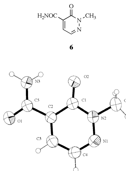
Figure 3. ORTEP [13] view of compound 6 displaying the thermal ellipsoids at 40% probability (for the sake of clarity only one molecule is showed)
