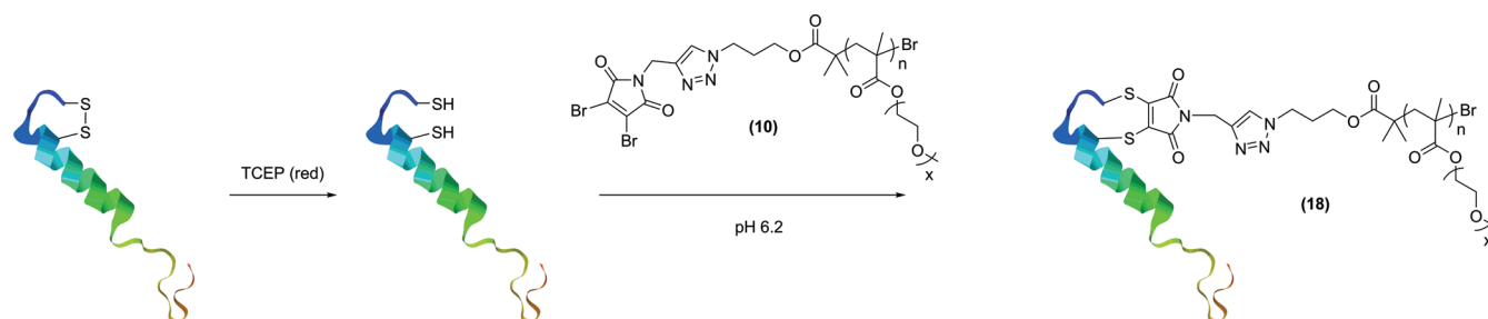
Figure 14. sCT disulfide rebridging using dibromomaleimide functional polymer 10.
