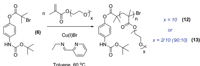
Figure 12. Polymerization of oligo(ethylene glycol) methacrylates using initiator 10 as a route to \alpha -Boc-protected polymers.
