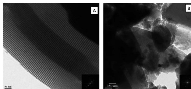
Fig. 6 TEM Images (A) calcined SBA-15 and (B) SBA-15-TAT-Pd(II).
