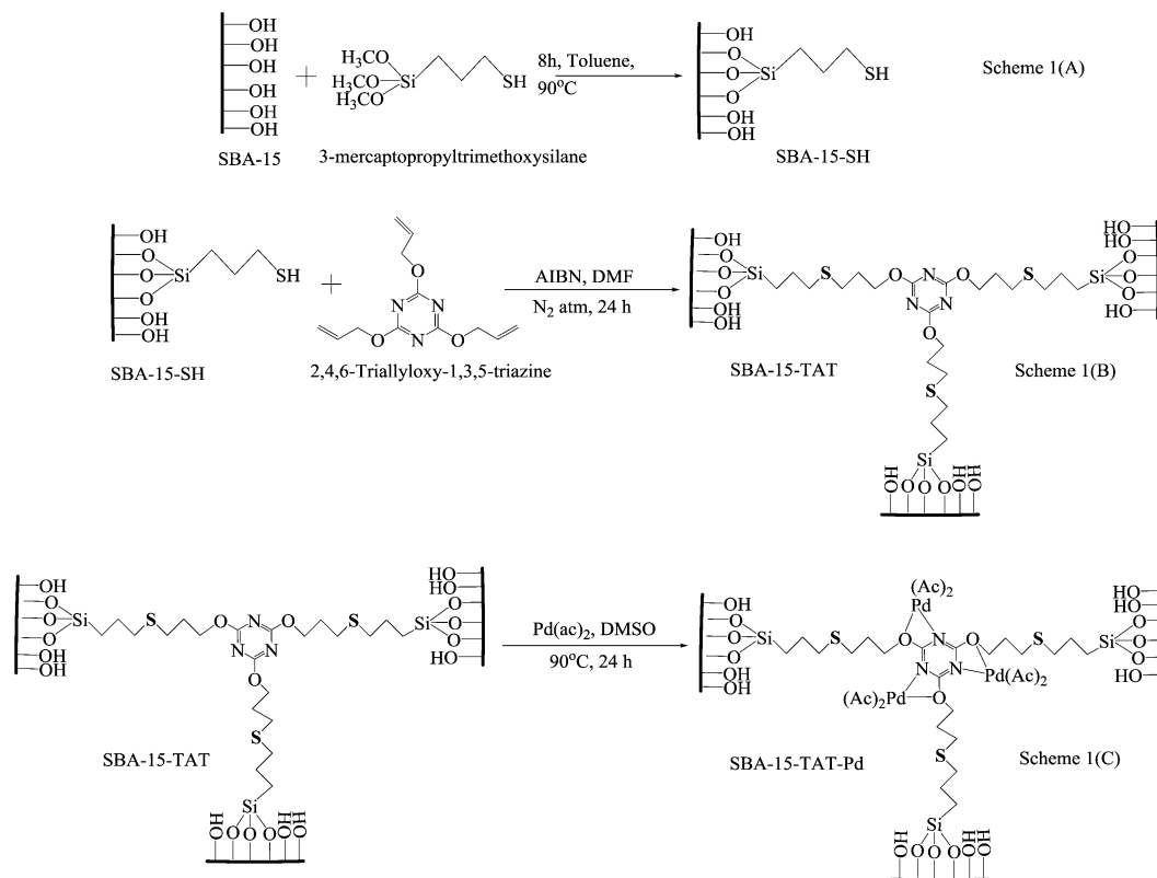
Scheme 1 Schematic diagram of heterogeneous SBA-15-TAT-Pd(II) synthesis. Surface Modification via 3-MPTMS (3-mercaptopropyl trimethoxysilane) of SBA-15, (B). Anchoring of 2,4,6-triallyloxy-1,3,5-triazine (TAT) complex over modified surface of SBA-15, (C). Metalation by Pd acetate.
