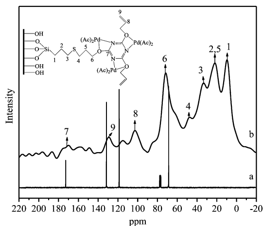
Fig. 4 Liquid ^{13}C NMR of (a) 2,4,6-triallyloxy-1,3,5-triazine (TAT) and (b) solid state ^{13}C CP MAS NMR of SBA-15-TAT-Pd(II).
