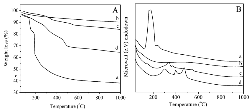
Fig. 8 (A) TGA, (B) DTA of (a) as-synthesized SBA-15, (b) calcined SBA-15, (c) SBA-15-SH and (d) SBA-15-TAT.
