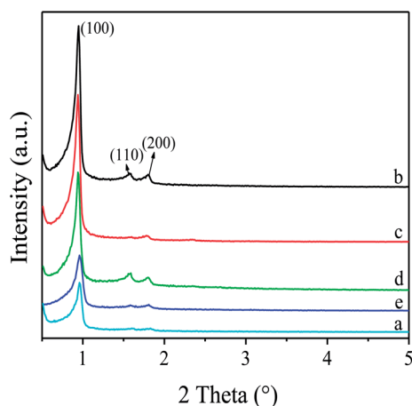
Fig. 1 XRD pattern of (a) as-synthesized SBA-15, (b) calcined SBA-15, (c) SBA-15-SH, (d) SBA-15-TAT, (e) SBA-15-TAT-Pd(II).
