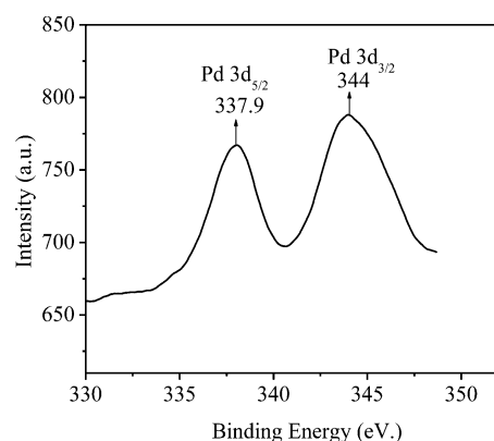
Fig. 10 XPS spectra of SBA-15–TAT–Pd(II).
