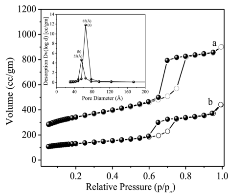
Fig. 9 Nitrogen adsorption–desorption isotherm and inset (BJH) pore size distribution of (a) calcined SBA-15 and (b) SBA-15–TAT–Pd(II).
