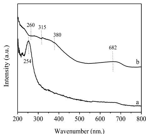
Fig. 3 UV-vis spectra of (a) calcined SBA-15 and (b) SBA-15-TAT-Pd(II).
