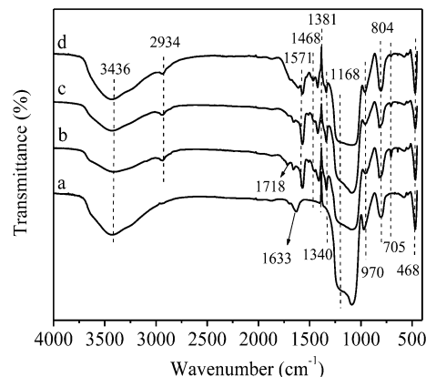
Fig. 2 FT-IR spectrum of (a) calcined SBA-15, (b) SBA-15-SH, (c) SBA-15-TAT and (d) SBA-15-TAT-Pd(II).
