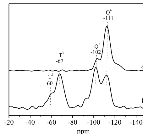
Fig. 5 Solid state ^{29}Si CP MAS NMR spectrum of (a) calcined SBA-15 and (b) SBA-15-TAT-Pd(II).
