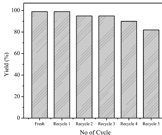
Fig. 11 Recycling study of heterogeneous catalyst SBA-15-TAT-Pd(II). Reaction conditions: 10 mmol of styrene, 150 psi of H 2 pressure, 0.025 g of catalyst SBA-15-TAT-Pd(II), 50 mL methanol, T = 40 °C.
