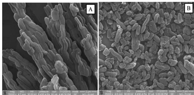
Fig. 7 SEM images of (A) calcined SBA-15 and (B) SBA-15-TAT-Pd(II).
