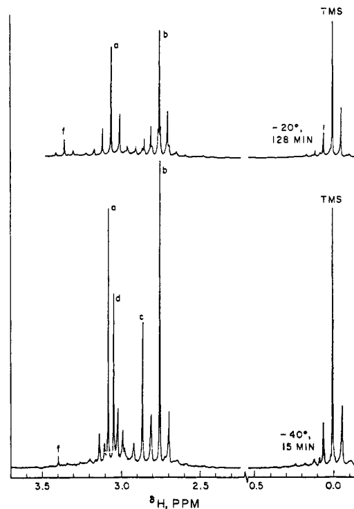
Figure 2. ^1\text{H} NMR spectrum of the product mixture from the MCPBA oxidation of S -methyl methanethiosulfinate (33) in \text{CDCl}_3 . The legend is the same as in Figure 1.
