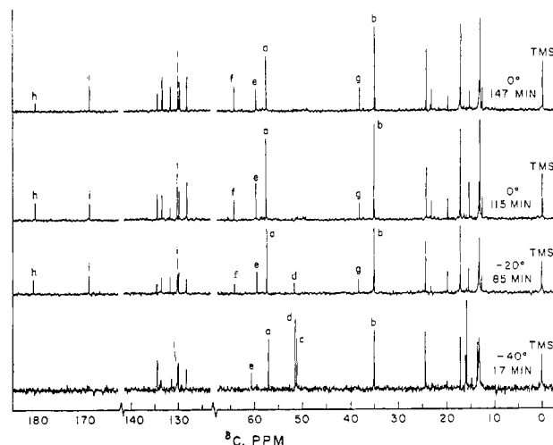
Figure 3. Temperature and time dependent ^1\text{H} NMR and ^{13}\text{C} NMR spectra of the products from the MCPBA oxidation of S -propyl propanethiosulfinate (34) in \text{CDCl}_3 .
