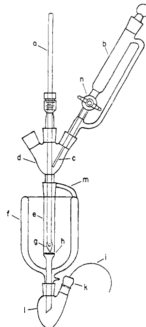
Figure 4. (a) Glass stirring rod; (b) addition funnel; (c) 1/8 -in. Teflon tube; (d) modified three-neck 25-mL flask; (e) 10-mL cylinder; (f) glass Dewar; (g) paddle; (h) medium glass frit; (i) 1/16 -in. Teflon tube; (k) septum; (l) two-neck 10-mL pear-shaped flask; (m) support rod; (n) Teflon stopper.
