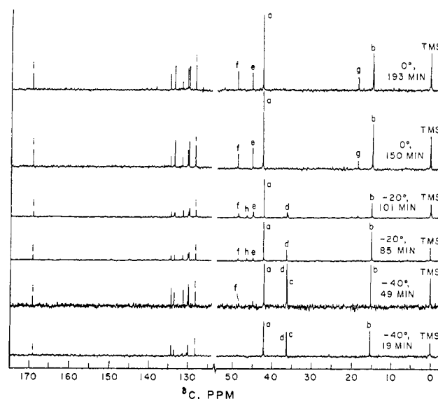
Figure 1. Temperature and time dependent 1 H NMR and 13 C NMR spectra of the products from the MCPBA oxidation of S -methyl methanethiosulfonate (33) in CDCl 3 .
