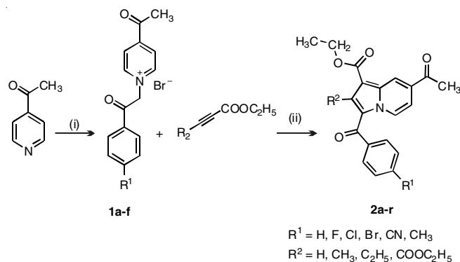
Scheme-I: Reagents and conditions: (i) 4-substituted phenacyl bromide, acetone, 5 h, stir; (ii) K_2CO_3 , DMF, 0.5 h stir at room temperature
