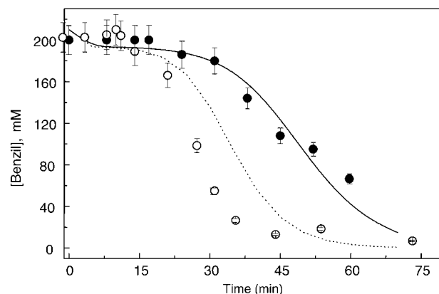
Figure 5. Reaction of lithium metal with benzil ( 1 ) in THF at 298 K; [\text{I}]_0 = 200 \text{ mM} . Circles are experimental data for the benzil decay under different initial lithium conditions: \text{Li} = 105 \text{ mg} , 12 pellets (●); \text{Li} = 400 \text{ mg} , 50 pellets (○). The broken line represents the simplified model prediction using the data in Table 1, with S proportional to the number of pellets ( S is reduced from 1 to 0.24). The solid line is a simulation using S = 0.24 and a slightly lower value of k_3 = 1.5 \times 10^{-4} \text{ s}^{-1} ; the rest of rate constants are as in Table 1
