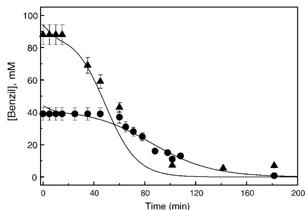
Figure 3. Reaction of lithium metal with benzil ( 1 ) in THF at 298 K, \text{Li} = 400 mg, at different benzil concentrations: [\text{1}]_0 = 88 mM ( \blacktriangle ) and 40 mM ( \bullet ); benzil decay as a function of time determined by GC analysis. Solid lines are the simulated concentration dependences derived from the numerical integration, according to the mechanism depicted in Scheme 1 and Table 1 (see the text)
