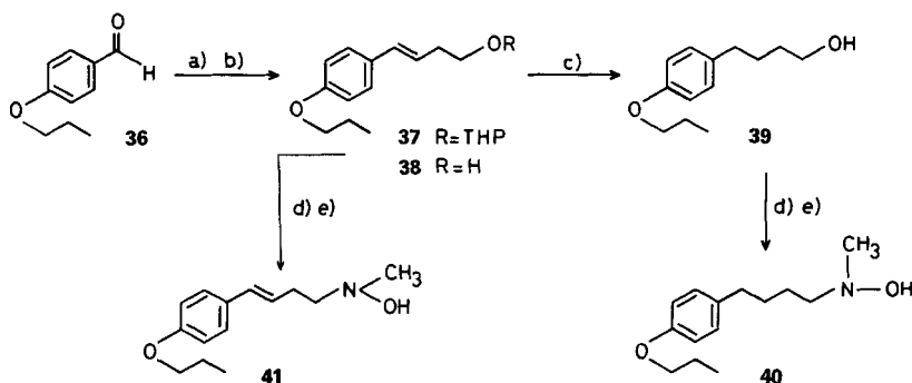
Scheme 6. Synthesis of N -[ (4-Alkoxyphenyl)alkyl or -alkenyl]hydroxylamines
