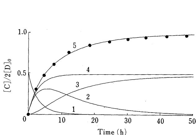
Fig. 2. Time Course of p -Nitrophenol Release from D at pH 10.0 and Analog Computer Simulation Curves of Hydrolysates of D
