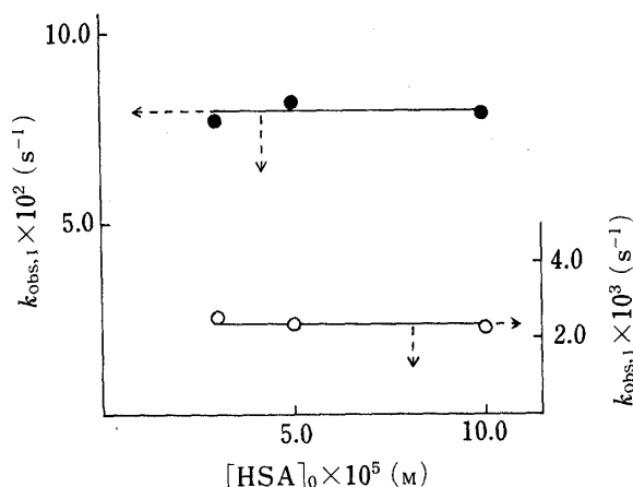
Fig. 6. Effect of HSA Concentration on k_{\text{obs},1} at 25 °C
