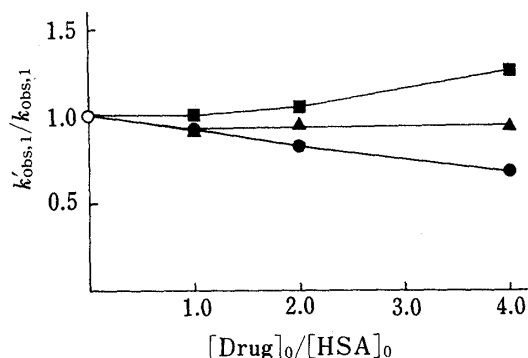
Fig. 4. Effects of U-Type Drugs on k_{\text{obs},1} at pH 7.4 and 25 °C
