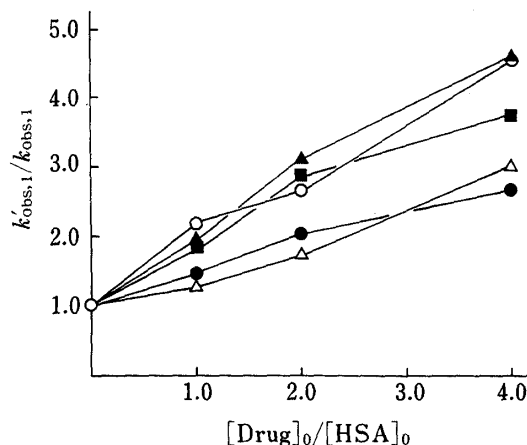
Fig. 5. Effects of R-Type Drugs on k_{\text{obs},1} at pH 7.4 and 25 °C
