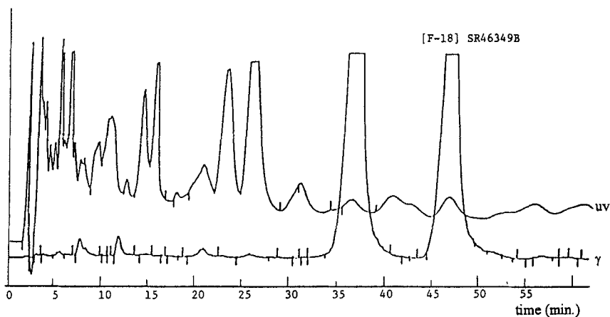
Figure 3 HPLC purification profile of [ ^{18}\text{F} ]SR46349B. Conditions: Econosil C-18 column (250 x 10 mm, 10 micron); solvent: MeOH:MeCN:0.1 M \text{K}_2\text{HPO}_4 = 27.5:27.5:45; flow rate = 5.0 ml/min.
