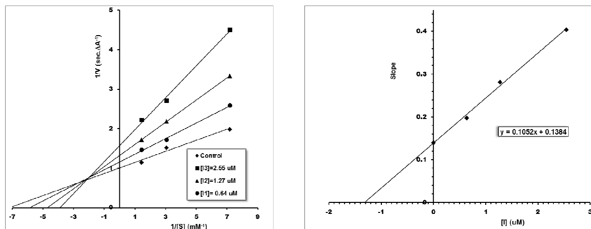
Figure 2. Left: Lineweaver-Burk plot for the inhibition of AChE by compound 4r at different concentrations of acetylthiocholine (ATCh), Right: Secondary plot of the enzyme for calculation of steady-state inhibition constant ( K_i = 1.32 \mu\text{M} ) of 4r .
