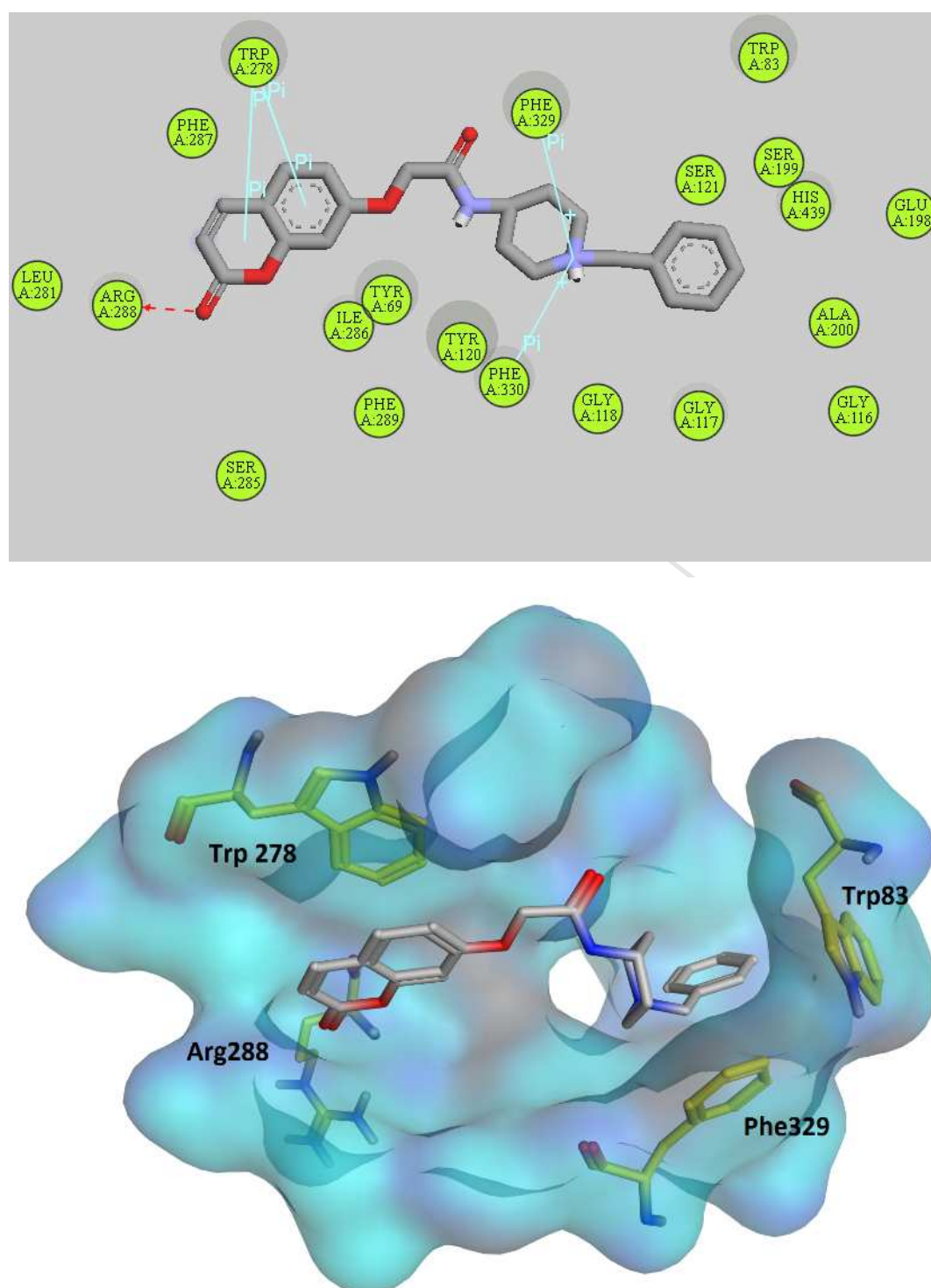
Figure 4. The schematic 2D and 3D representations (top and bottom, respectively) of compound 4r, docked in the active site of AChE.
