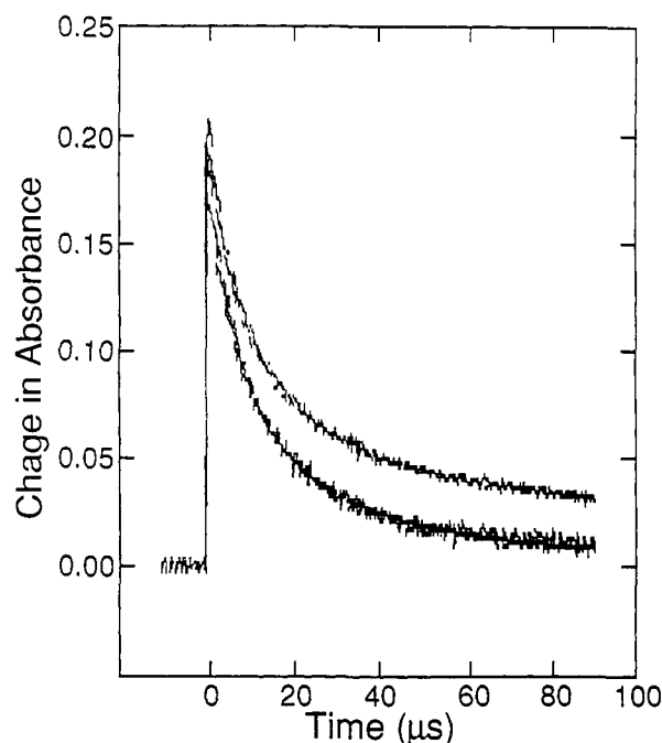
Figure 4. Time dependence of the absorption of the ethyl viologen radical cation (EV •+ , upper trace) and the DEBP •+ radical cation (lower trace) following laser irradiation of the acetylantanthracene sensitizer. The data are the individual points; the (barely visible) solid line is the least-squares fit according to the kinetic model described in the text.
