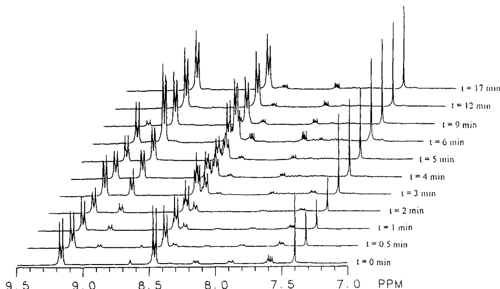
Figure 2. A portion of the ^1\text{H} NMR spectrum of the \text{N}_2 -saturated acetonitrile solution of acetylanthracene and \text{DEBP}^{2+} , recorded during the photochemical sensitization of \text{DEBP}^{2+} with acetylanthracene in \text{CD}_3\text{CN} solution.
