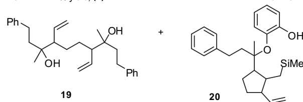
Scheme 11. Reactions of Bistro 1 with 4-phenylbutan-2-one derivatives.
