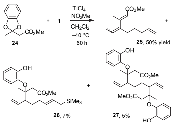
Scheme 16. Reaction of Bistro with methyl acetylacate catechol ketal 24 .
