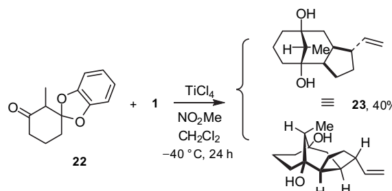
Scheme 13. Reaction of Bistro 1 with 2-methylcyclohexan-1,3-dione mono catechol ketal 22 .
