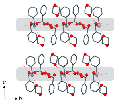
Figure 5. Crystal structure of 2((+)-1)·(–)-2·2(1,4-dioxane) viewed from the a axis. Hydrogen atoms are omitted for clarity. The dotted lines and shadows represent hydrogen bonds and hydrogen-bonding networks, respectively.
