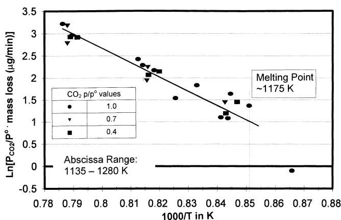
Fig. 5. Volatile weight loss from \text{K}_2\text{CO}_3 during thermal analysis at elevated temperatures. The effect of \text{CO}_2 partial pressure on decomposition.
