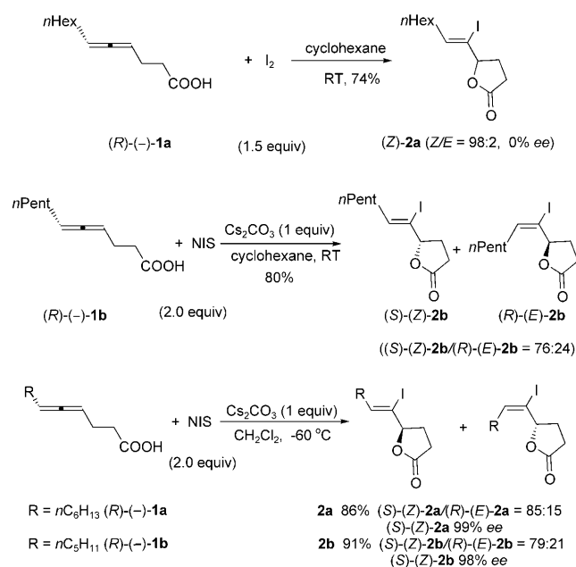
Scheme 2. Intramolecular iodolactonization of optically active 4,5-allenoic acids ( R )-(-)- 1a and ( R )-(-)- 1b with \text{I}_2 or NIS. NIS = N -iodosuccinimide.
