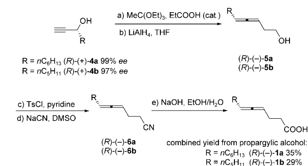
Scheme 1. Synthesis of optically active \gamma -allenoic acids ( R )-(-)- 1a and ( R )-(-)- 1b . Ts = tosyl.
