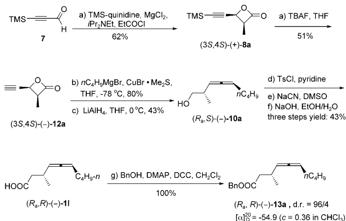
Scheme 7. Synthesis of optically active \gamma -allenoic acid ( R a , R )-(-)- 11 . DCC=1,3-dicyclohexylcarbodiimide; DMAP=4-dimethylaminopyridine.
