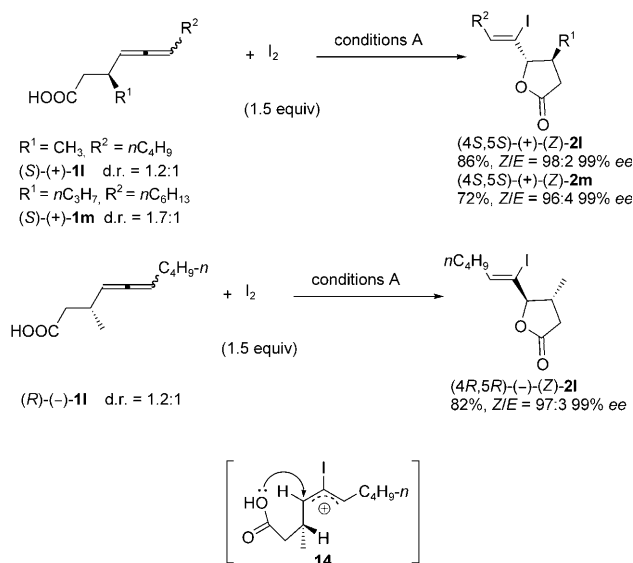
Scheme 6. Iodolactonization of optically active 4,5-allenoic acids ( S )-(+)- 11 , ( S )-(+)- 1m , and ( R )-(-)- 11 with \text{I}_2 .
