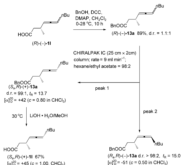
Scheme 8. Synthesis of optically active \gamma -allenoic acids ( S a , R )-(+)- 11 .
