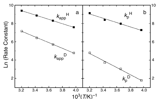
Fig. 3 Arrhenius plots for the reactions of \text{DMA}^{+\bullet} (solid squares) and \text{DMA-d}_6^{+\bullet} (open squares) with LUT in acetonitrile- \text{Bu}_4\text{NPF}_6 (0.1 M) derived from apparent rate constants (a) and microscopic rate constants (b).
