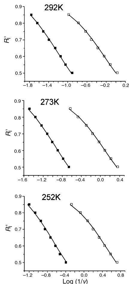
Fig. 2 DCV kinetic data for the reactions of \text{DMA}^{+\bullet} (solid squares) and \text{DMA-d}_6^{+\bullet} (open squares) with DEP in dichloromethane- \text{Bu}_4\text{NPF}_6 (0.2 M) as a function of temperature. The solid lines represent theoretical data for the complex proton transfer mechanism.
