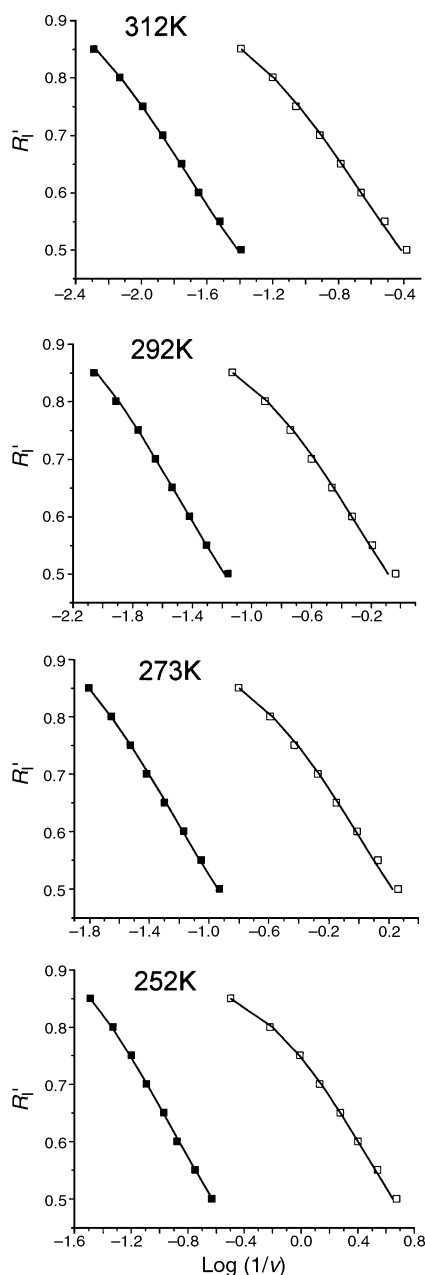
Fig. 1 DCV kinetic data for the reactions of \text{DMA}^{+\bullet} (solid squares) and \text{DMA-d}_6^{+\bullet} (open squares) with LUT in acetonitrile- \text{Bu}_4\text{NPF}_6 (0.1 M) as a function of temperature. The solid lines represent theoretical data for the complex proton transfer mechanism.
