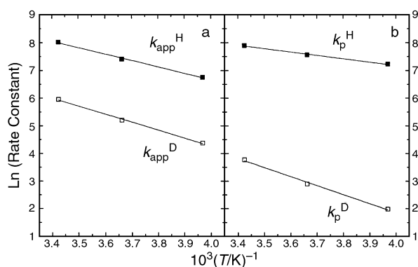
Fig. 4 Arrhenius plots for the reactions of DMA + • (solid squares) and DMA-d 6 + • (open squares) with DEP in acetonitrile-Bu 4 NPF 6 (0.1 M) derived from apparent rate constants (a) and microscopic rate constants (b).
