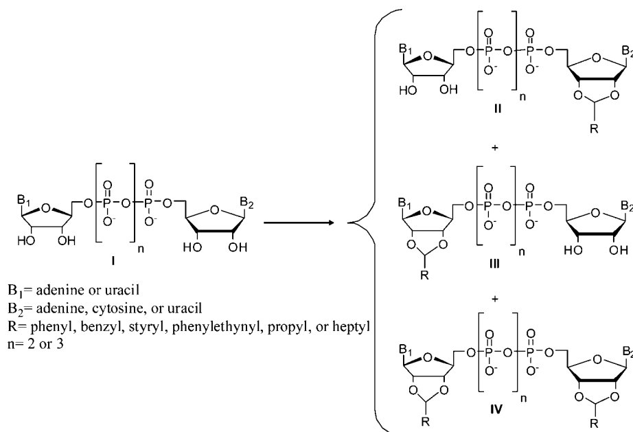
Scheme 2. Synthesis of Diadenosine Tetraphosphate and Adenosine Analogues a
