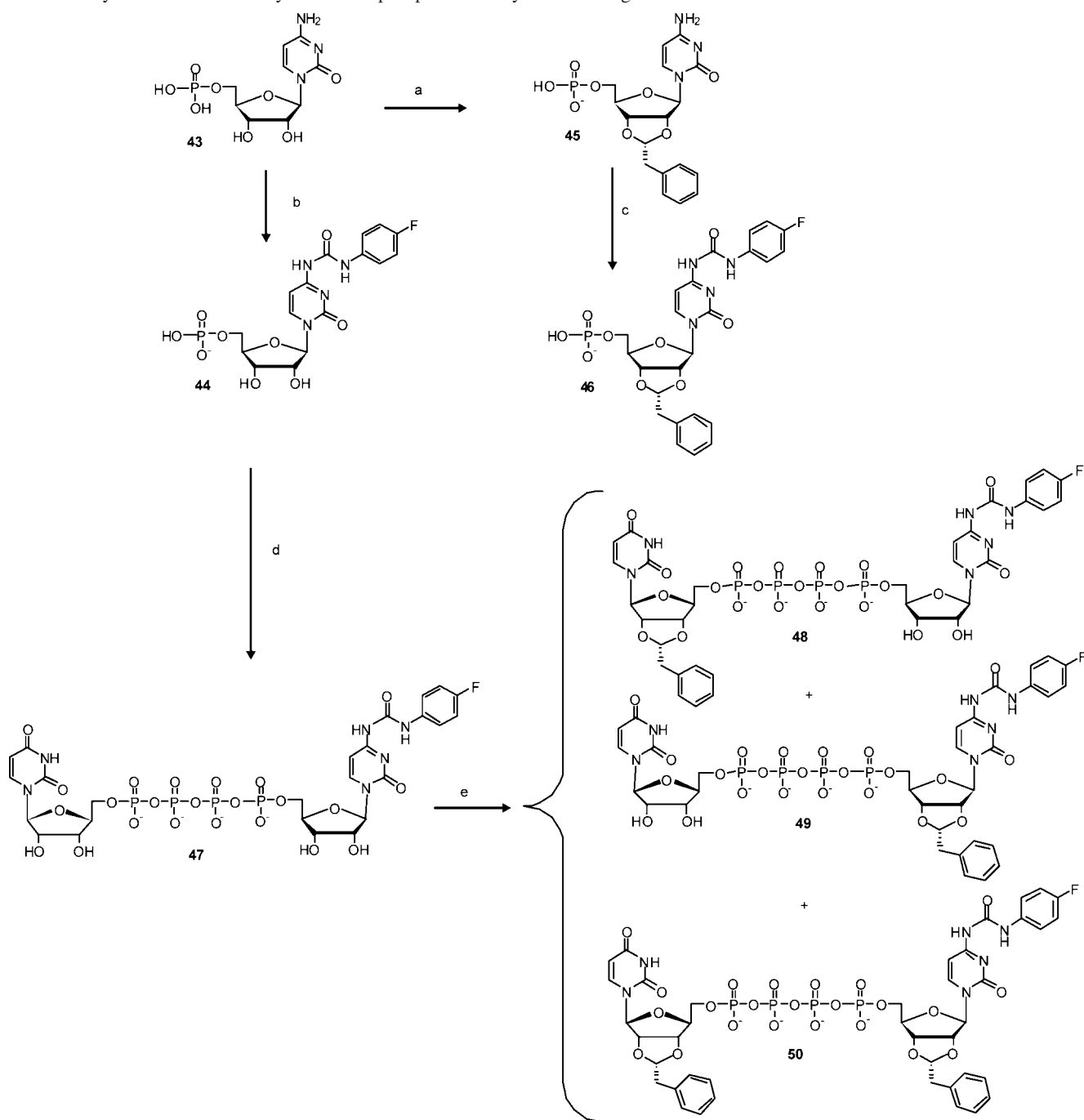
Scheme 3. Synthesis of Uridine Cytidine Tetraphosphate and Cytidine Analogues a
