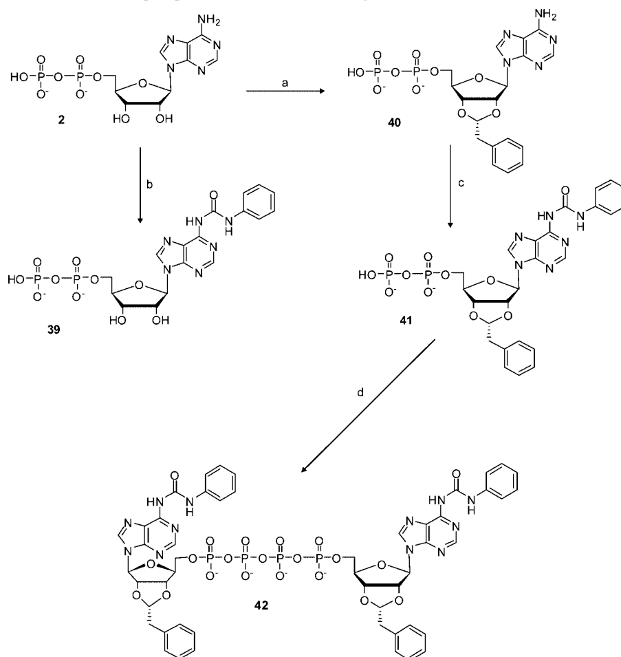
Scheme 2. Synthesis of Diadenosine Tetraphosphate and Adenosine Analogues a
