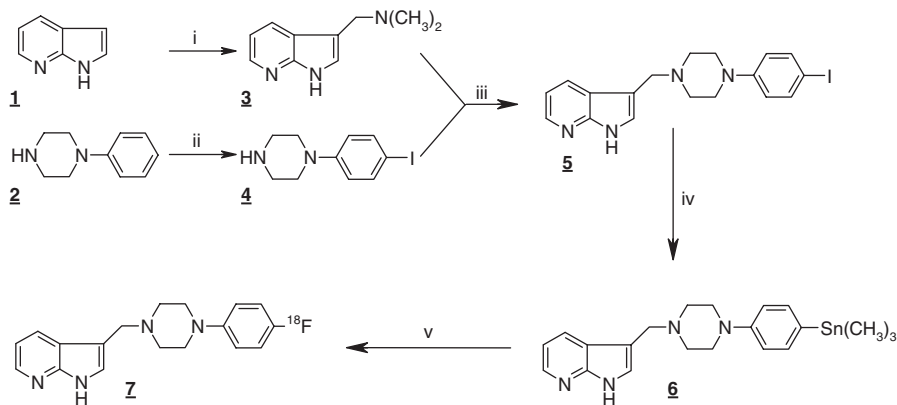
Figure 2. Synthesis of the stannylated precursor 6 and the radioligand [ ^{18}\text{F} ]F5P 7 : (i) dimethylammoniumchloride, paraformaldehyde, butanol, \Delta ; (ii) \text{ICl} , \text{AcOH}/\text{H}_2\text{O} ( 3 / 1 ), 60^\circ\text{C} ; (iii) xylene, \Delta ; (iv) \text{Sn}_2(\text{CH}_3)_6 , (\text{PPh}_3)_4\text{Pd}(0) , dioxane, \Delta ; and (v) \text{CCl}_3\text{F} , \text{AcOH} , [ ^{18}\text{F} ]F _2 .
