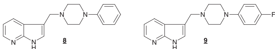
Figure 3. Structural formulae of compounds 8 , the major chemical impurity generated in labelling synthesis, and 9 , the reference compound
